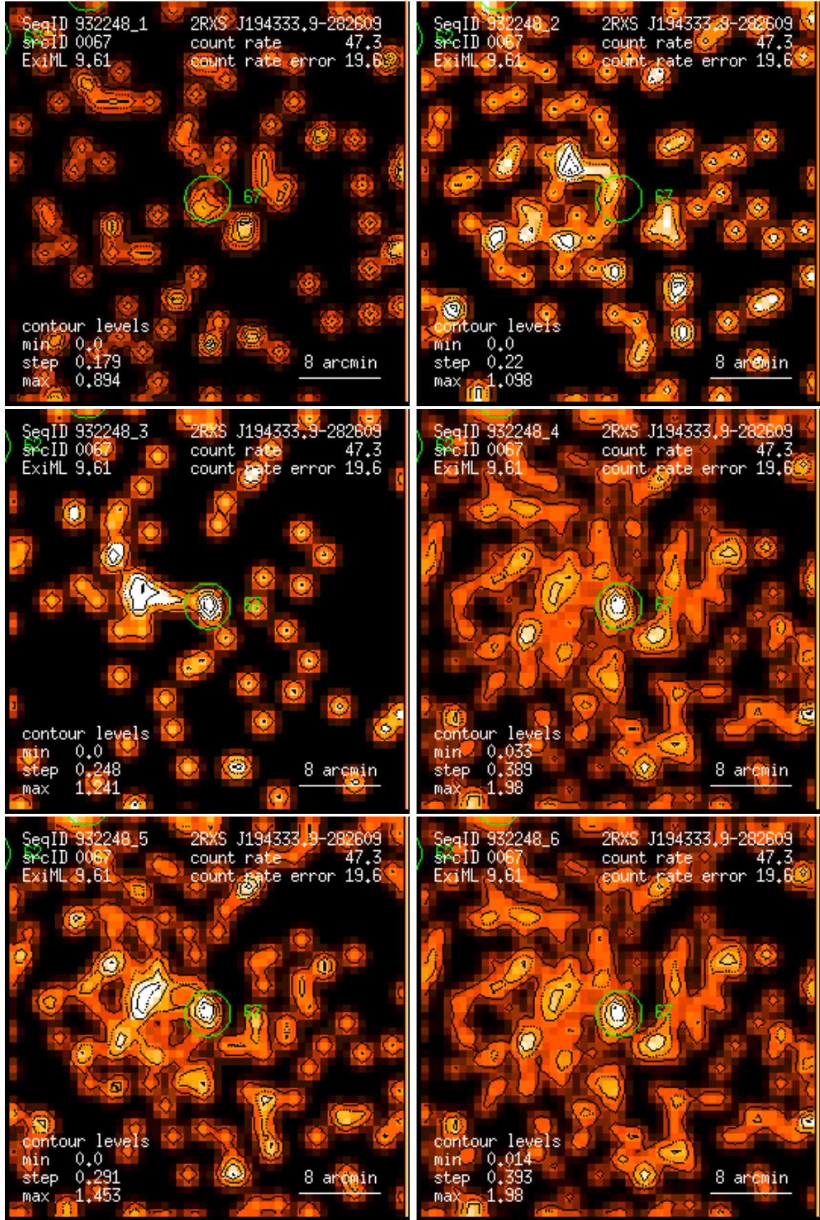
Figure 67: RASS 932248: detection 0067: band rate images, Gaussian filter: (1) PSPC channels 11 – 41, (2) 52 – 90, (3) 91 – 201, (4) 11 – 235, (5) 52 – 201, (6) 11 – 201. Broad band rates in counts/ks. Band rate contour levels in counts/ks/arcmin 2 .
