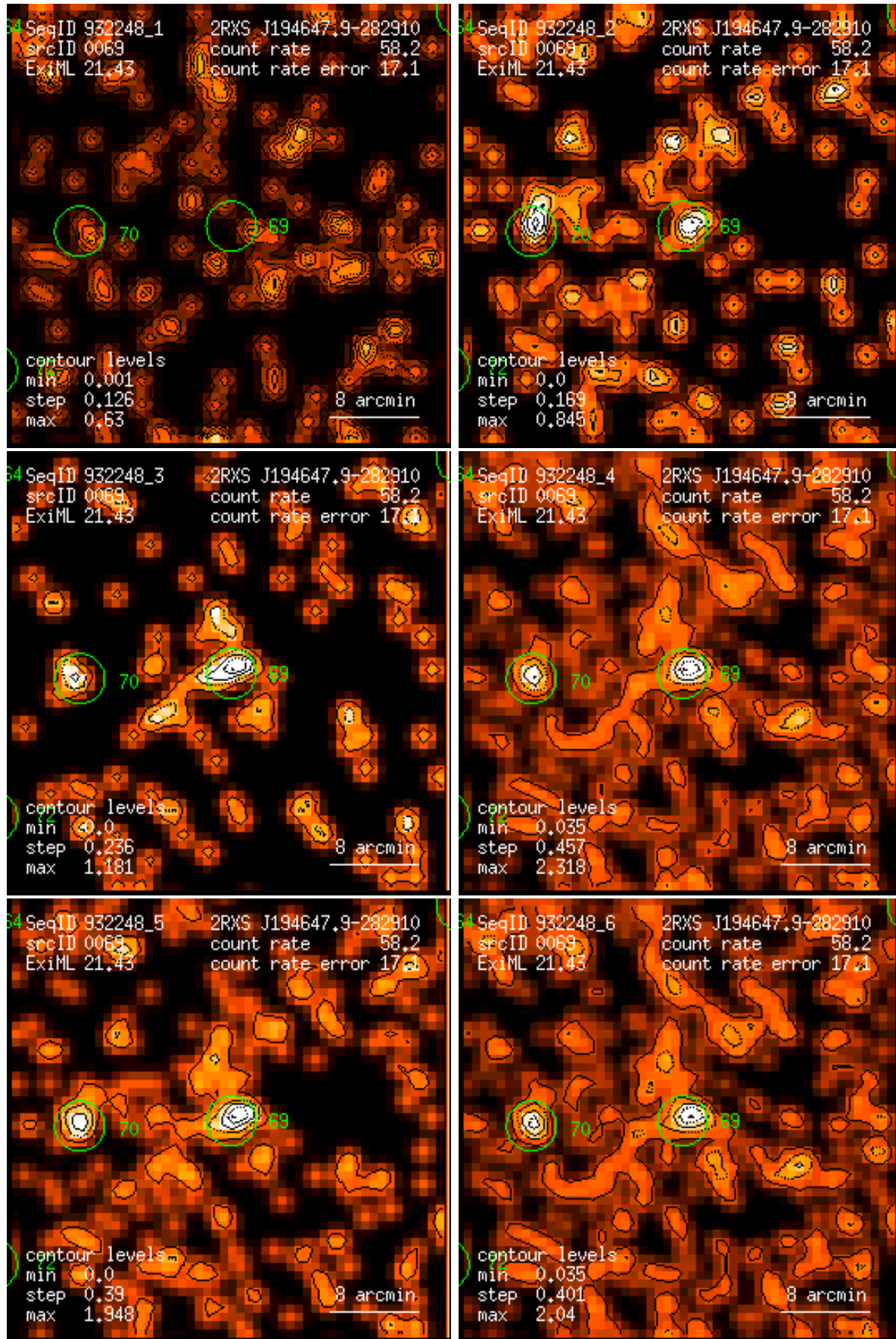
Figure 69: RASS 932248: detection 0069: band rate images, Gaussian filter: (1) PSPC channels 11 – 41, (2) 52 – 90, (3) 91 – 201, (4) 11 – 235, (5) 52 – 201, (6) 11 – 201. Broad band rates in counts/ks. Band rate contour levels in counts/ks/arcmin 2 .
