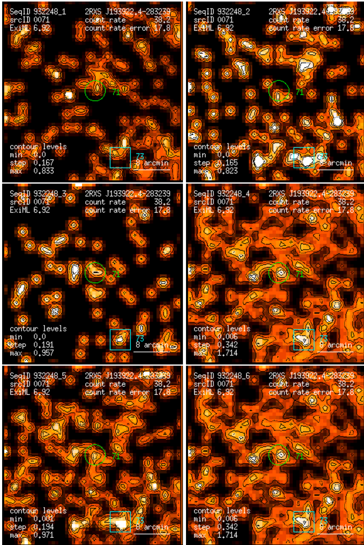
Figure 71: RASS 932248: detection 0071: band rate images, Gaussian filter: (1) PSPC channels 11 – 41, (2) 52 – 90, (3) 91 – 201, (4) 11 – 235, (5) 52 – 201, (6) 11 – 201. Broad band rates in counts/ks. Band rate contour levels in counts/ks/arcmin 2 .
