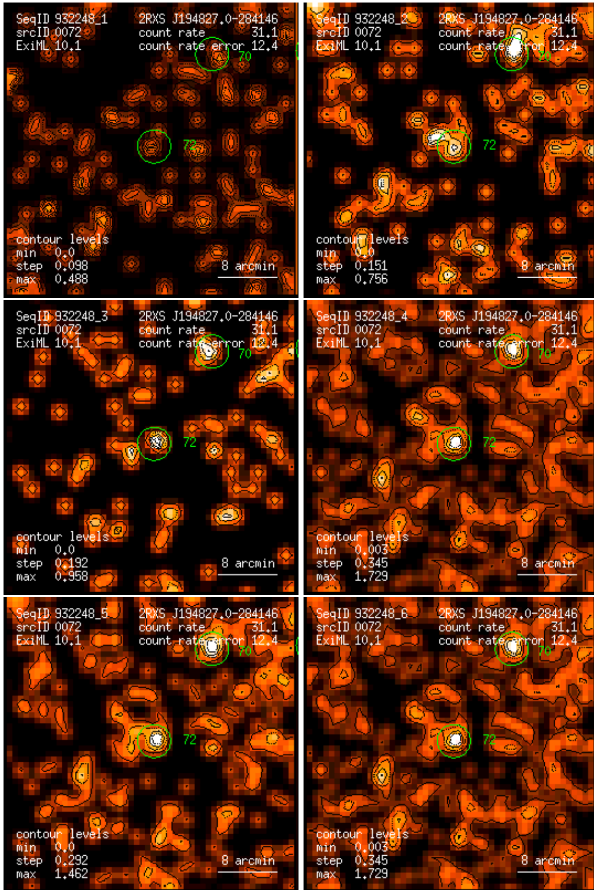
Figure 72: RASS 932248: detection 0072: band rate images, Gaussian filter: (1) PSPC channels 11 – 41, (2) 52 – 90, (3) 91 – 201, (4) 11 – 235, (5) 52 – 201, (6) 11 – 201. Broad band rates in counts/ks. Band rate contour levels in counts/ks/arcmin 2 .
