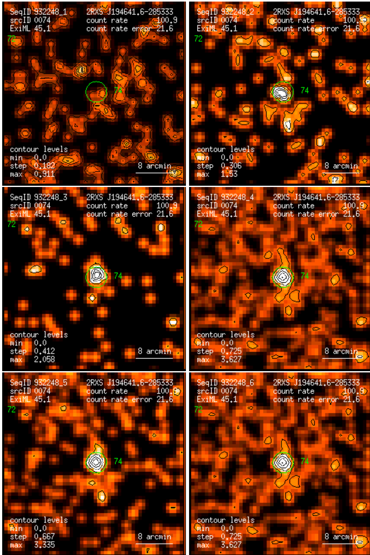
Figure 74: RASS 932248: detection 0074: band rate images, Gaussian filter: (1) PSPC channels 11 – 41, (2) 52 – 90, (3) 91 – 201, (4) 11 – 235, (5) 52 – 201, (6) 11 – 201. Broad band rates in counts/ks. Band rate contour levels in counts/ks/arcmin 2 .
