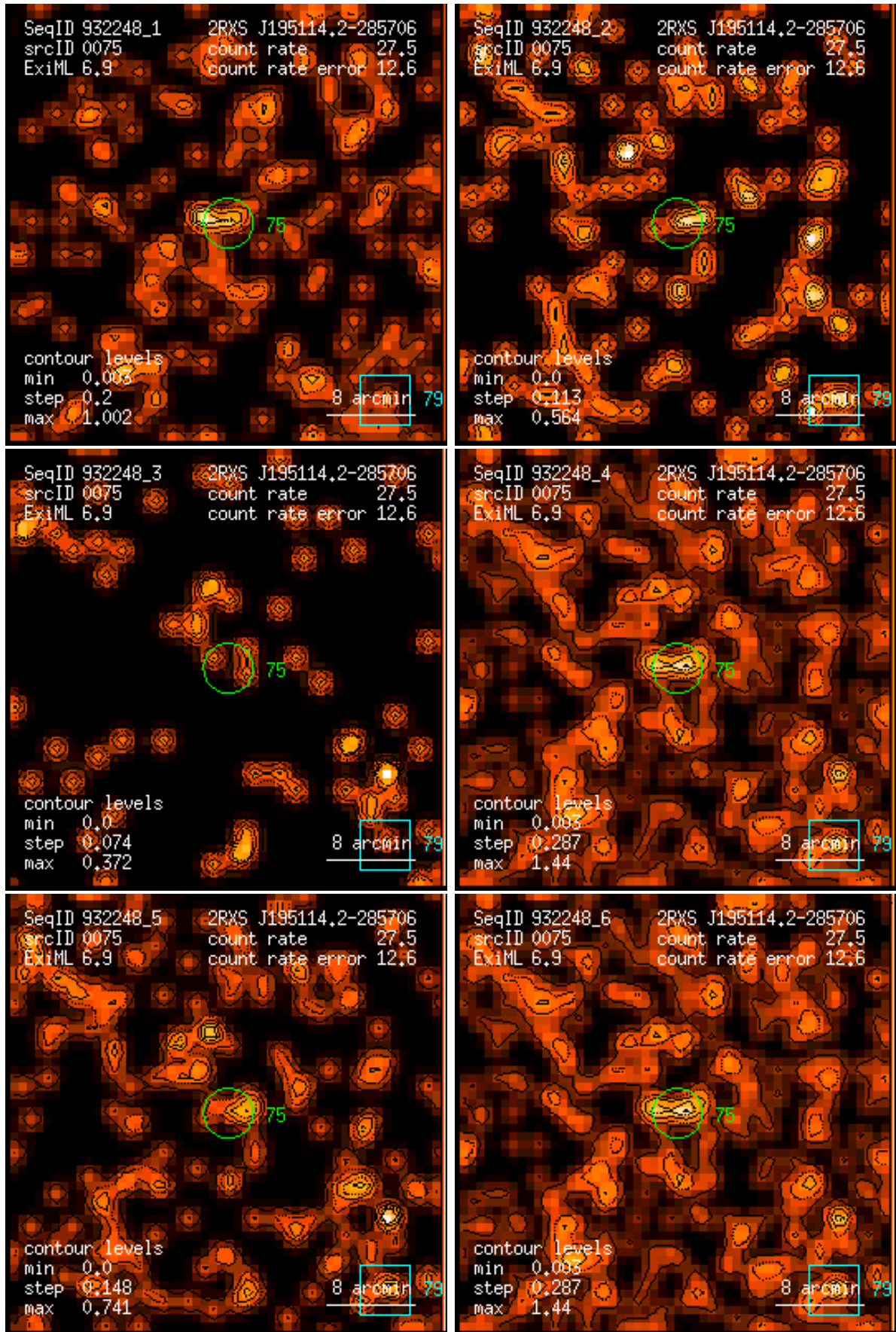
Figure 75: RASS 932248: detection 0075: band rate images, Gaussian filter: (1) PSPC channels 11 – 41, (2) 52 – 90, (3) 91 – 201, (4) 11 – 235, (5) 52 – 201, (6) 11 – 201. Broad band rates in counts/ks. Band rate contour levels in counts/ks/arcmin 2 .
