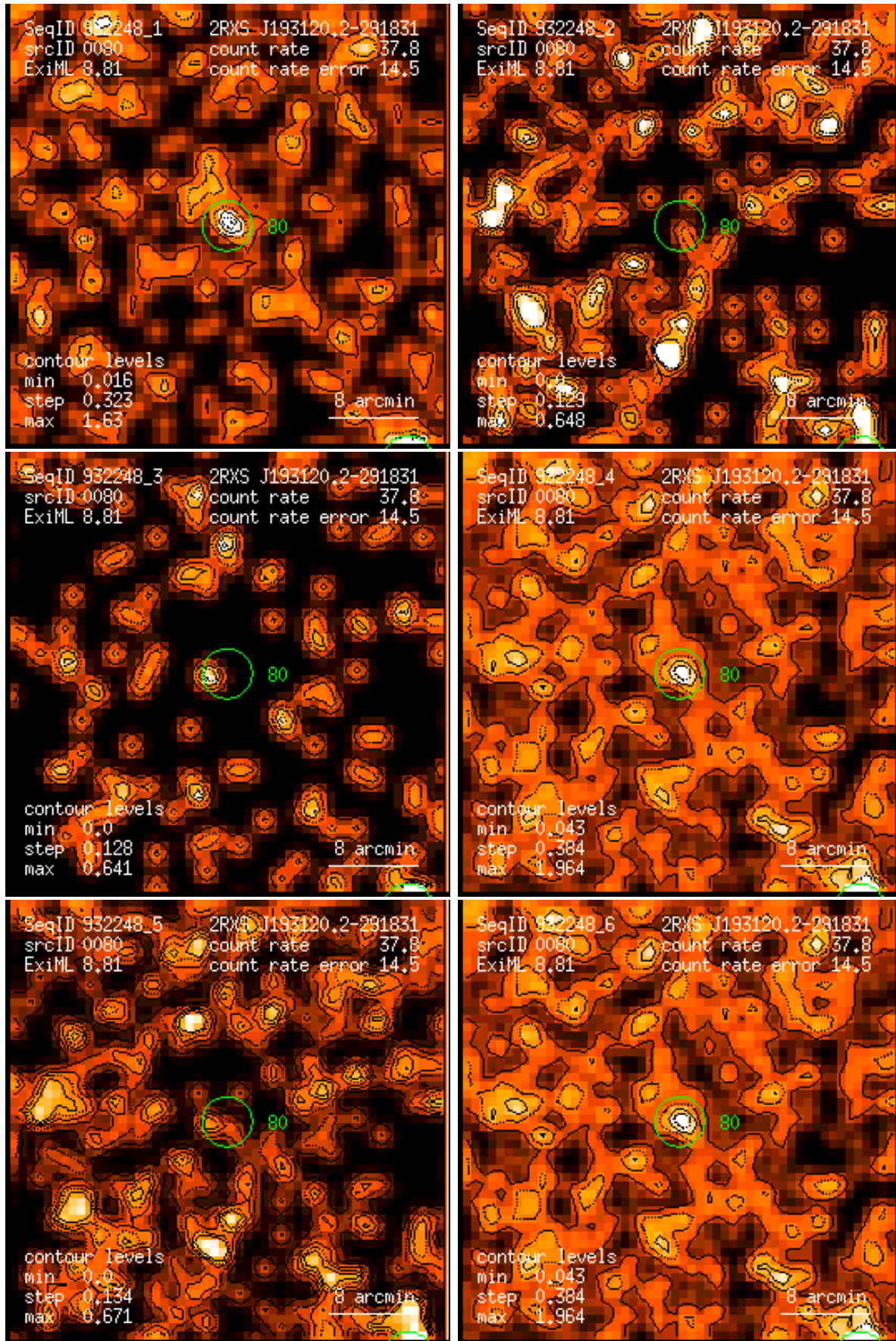
Figure 80: RASS 932248: detection 0080: band rate images, Gaussian filter: (1) PSPC channels 11 – 41, (2) 52 – 90, (3) 91 – 201, (4) 11 – 235, (5) 52 – 201, (6) 11 – 201. Broad band rates in counts/ks. Band rate contour levels in counts/ks/arcmin 2 .
