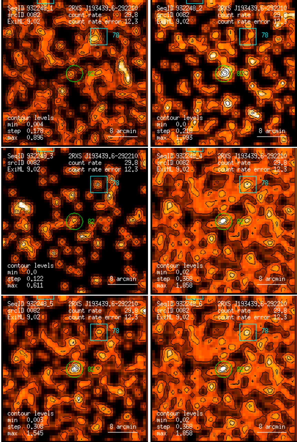
Figure 82: RASS 932248: detection 0082: band rate images, Gaussian filter: (1) PSPC channels 11 – 41, (2) 52 – 90, (3) 91 – 201, (4) 11 – 235, (5) 52 – 201, (6) 11 – 201. Broad band rates in counts/ks. Band rate contour levels in counts/ks/arcmin 2 .
