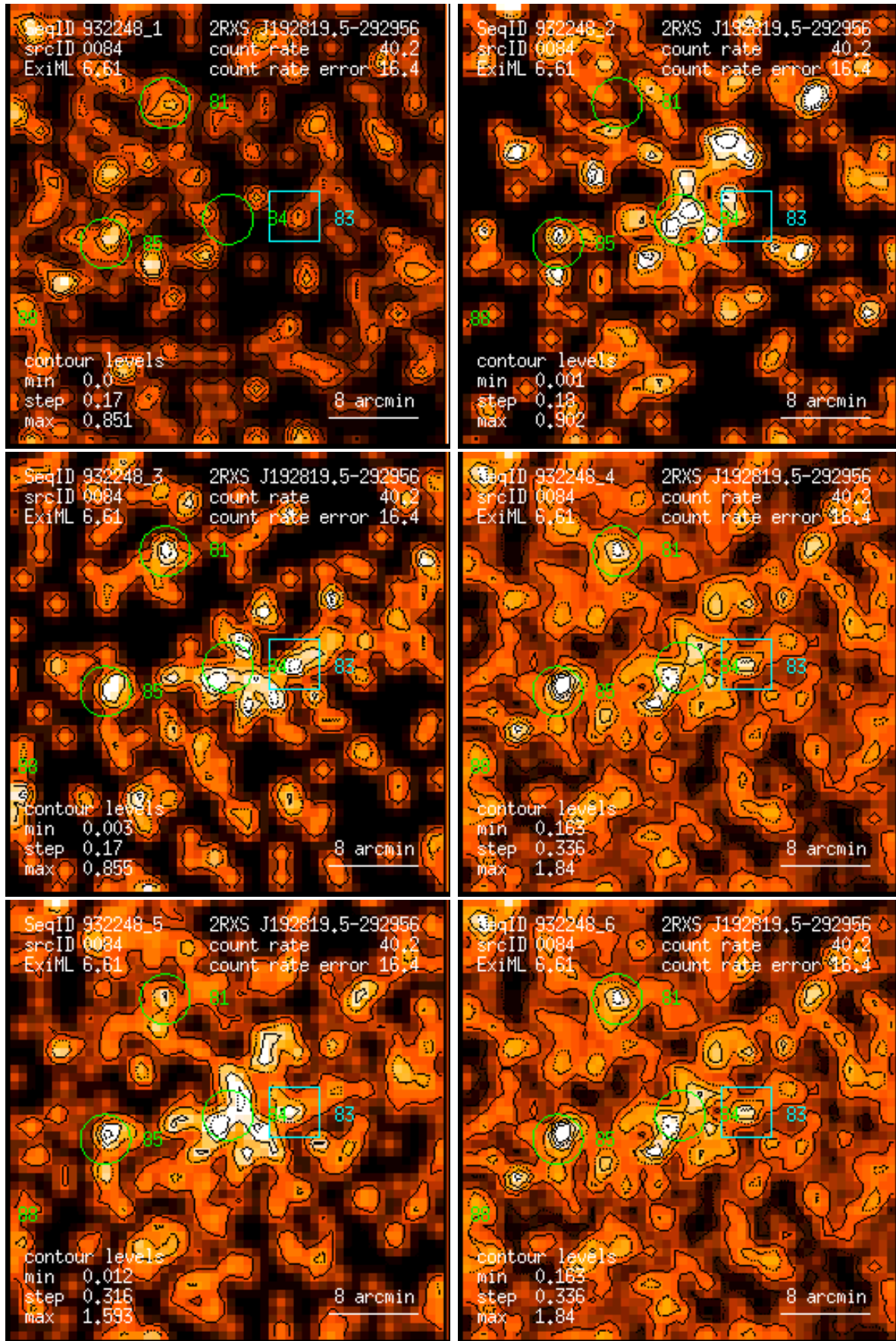
Figure 84: RASS 932248: detection 0084: band rate images, Gaussian filter: (1) PSPC channels 11 – 41, (2) 52 – 90, (3) 91 – 201, (4) 11 – 235, (5) 52 – 201, (6) 11 – 201. Broad band rates in counts/ks. Band rate contour levels in counts/ks/arcmin 2 .
