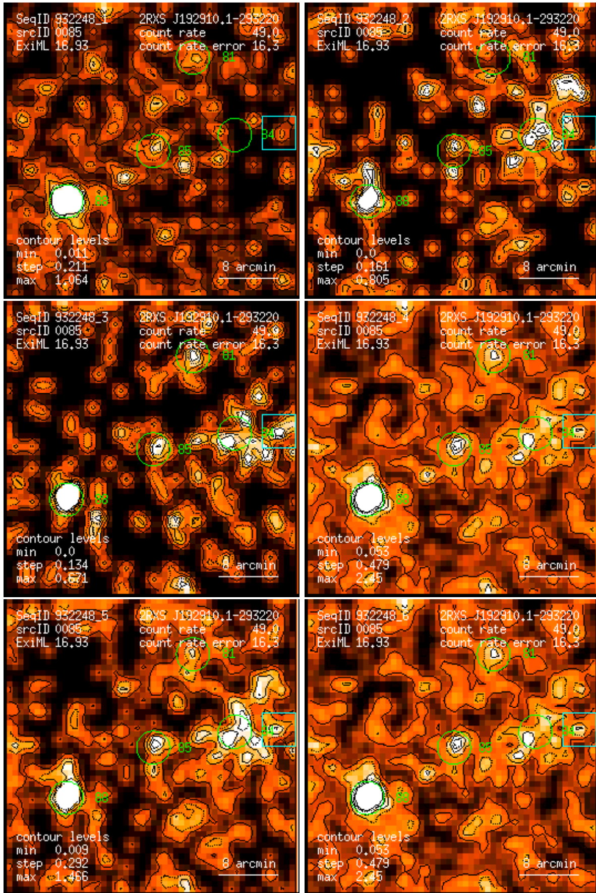
Figure 85: RASS 932248: detection 0085: band rate images, Gaussian filter: (1) PSPC channels 11 – 41, (2) 52 – 90, (3) 91 – 201, (4) 11 – 235, (5) 52 – 201, (6) 11 – 201. Broad band rates in counts/ks. Band rate contour levels in counts/ks/arcmin 2 .
