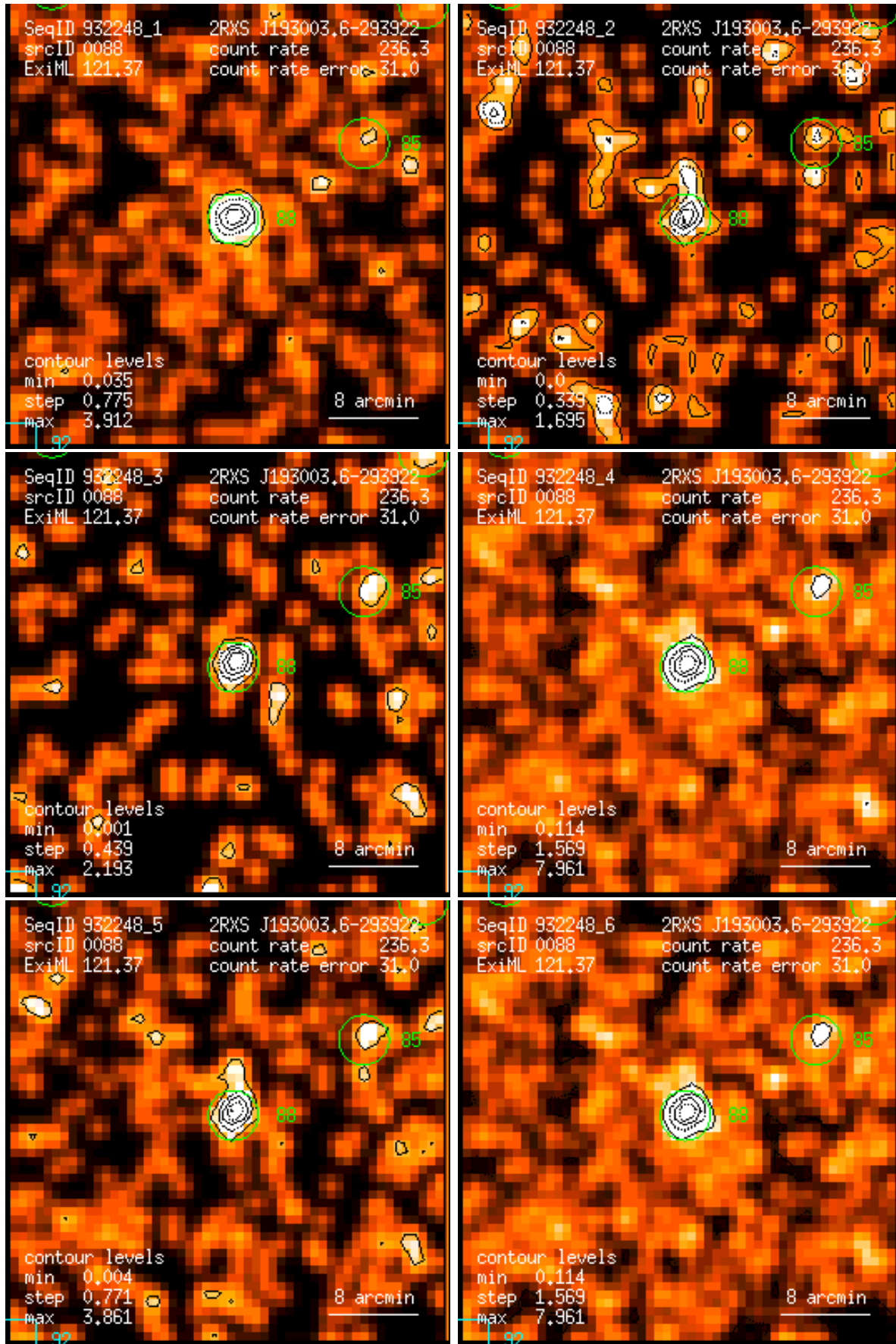
Figure 88: RASS 932248: detection 0088: band rate images, Gaussian filter: (1) PSPC channels 11 – 41, (2) 52 – 90, (3) 91 – 201, (4) 11 – 235, (5) 52 – 201, (6) 11 – 201. Broad band rates in counts/ks. Band rate contour levels in counts/ks/arcmin 2 .
