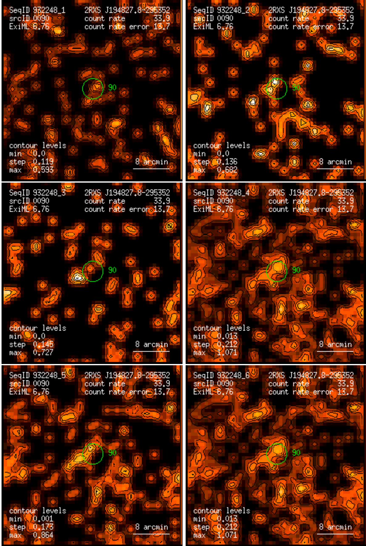
Figure 90: RASS 932248: detection 0090: band rate images, Gaussian filter: (1) PSPC channels 11 – 41, (2) 52 – 90, (3) 91 – 201, (4) 11 – 235, (5) 52 – 201, (6) 11 – 201. Broad band rates in counts/ks. Band rate contour levels in counts/ks/arcmin 2 .
