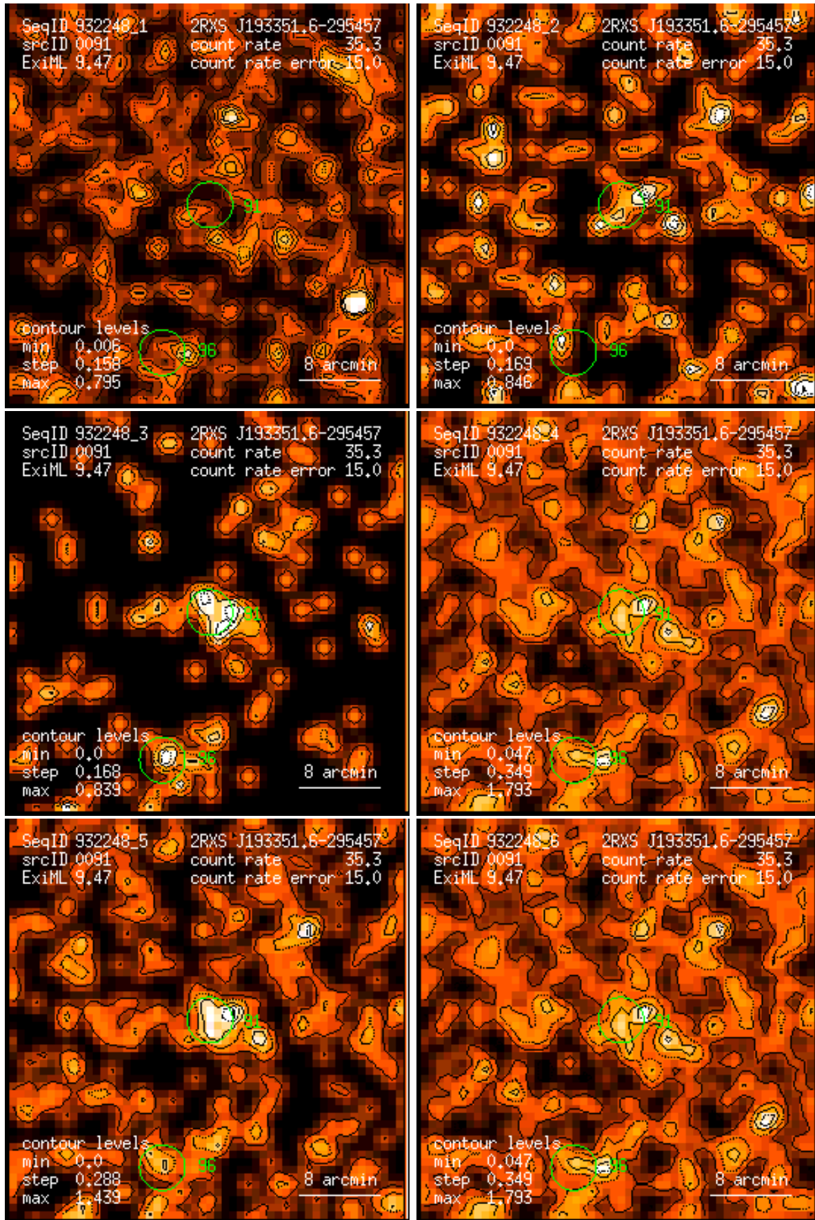
Figure 91: RASS 932248: detection 0091: band rate images, Gaussian filter: (1) PSPC channels 11 – 41, (2) 52 – 90, (3) 91 – 201, (4) 11 – 235, (5) 52 – 201, (6) 11 – 201. Broad band rates in counts/ks. Band rate contour levels in counts/ks/arcmin 2 .
