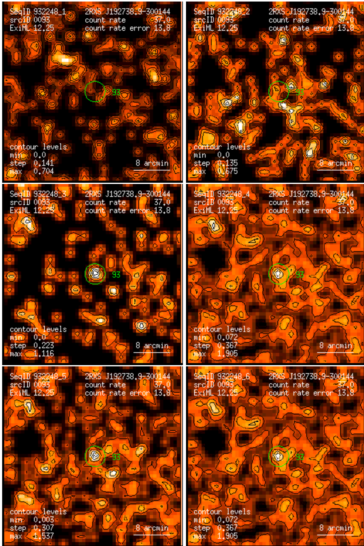
Figure 93: RASS 932248: detection 0093: band rate images, Gaussian filter: (1) PSPC channels 11 – 41, (2) 52 – 90, (3) 91 – 201, (4) 11 – 235, (5) 52 – 201, (6) 11 – 201. Broad band rates in counts/ks. Band rate contour levels in counts/ks/arcmin 2 .
