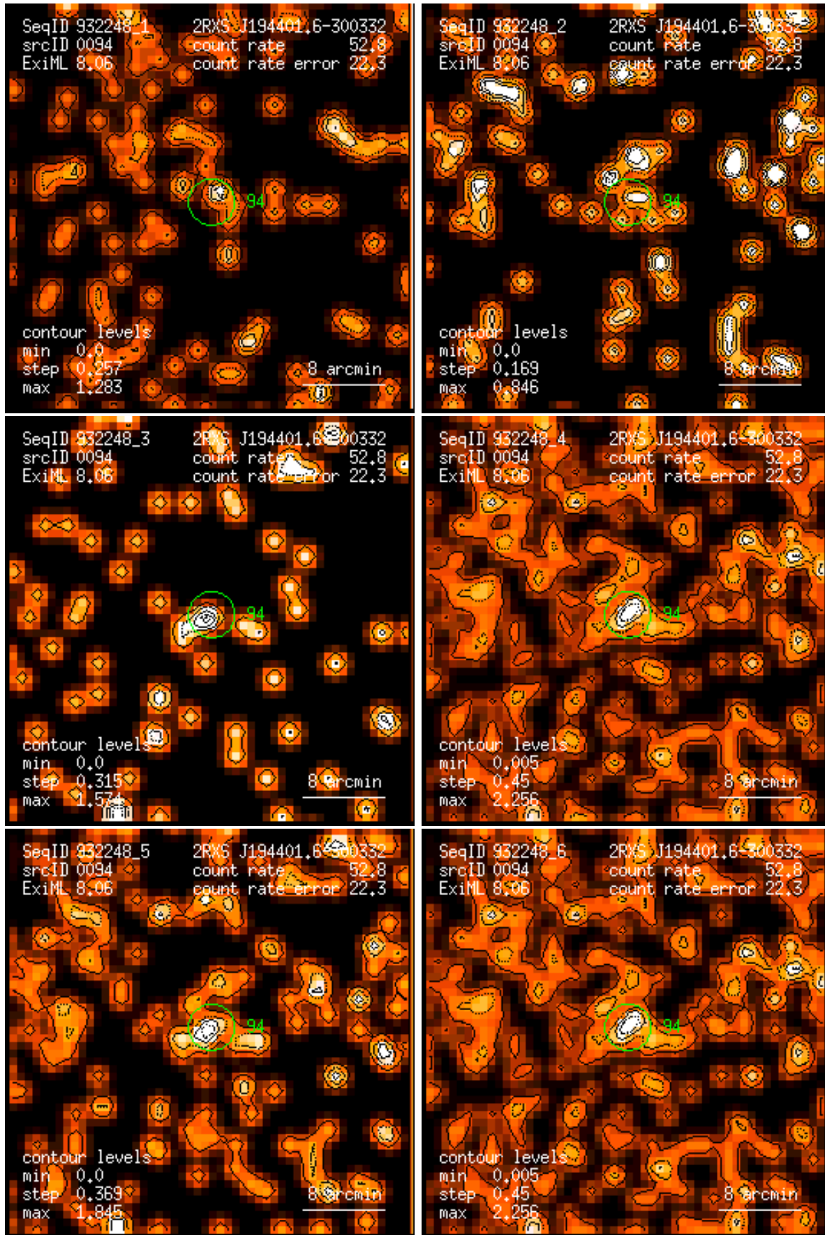
Figure 94: RASS 932248: detection 0094: band rate images, Gaussian filter: (1) PSPC channels 11 – 41, (2) 52 – 90, (3) 91 – 201, (4) 11 – 235, (5) 52 – 201, (6) 11 – 201. Broad band rates in counts/ks. Band rate contour levels in counts/ks/arcmin 2 .
