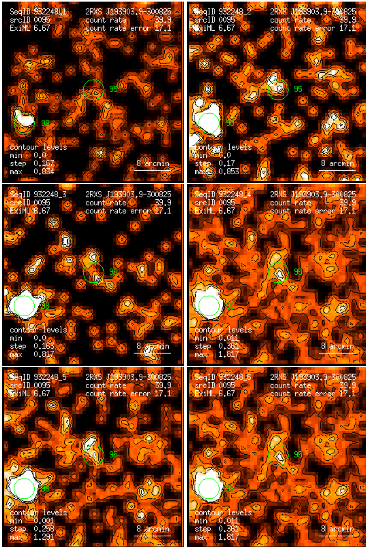
Figure 95: RASS 932248: detection 0095: band rate images, Gaussian filter: (1) PSPC channels 11 – 41, (2) 52 – 90, (3) 91 – 201, (4) 11 – 235, (5) 52 – 201, (6) 11 – 201. Broad band rates in counts/ks. Band rate contour levels in counts/ks/arcmin 2 .
