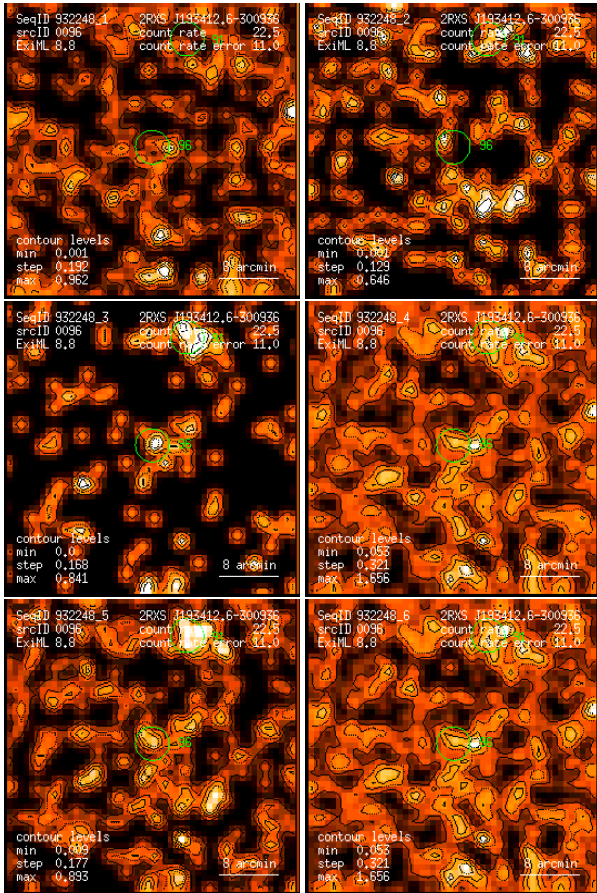
Figure 96: RASS 932248: detection 0096: band rate images, Gaussian filter: (1) PSPC channels 11 – 41, (2) 52 – 90, (3) 91 – 201, (4) 11 – 235, (5) 52 – 201, (6) 11 – 201. Broad band rates in counts/ks. Band rate contour levels in counts/ks/arcmin 2 .
