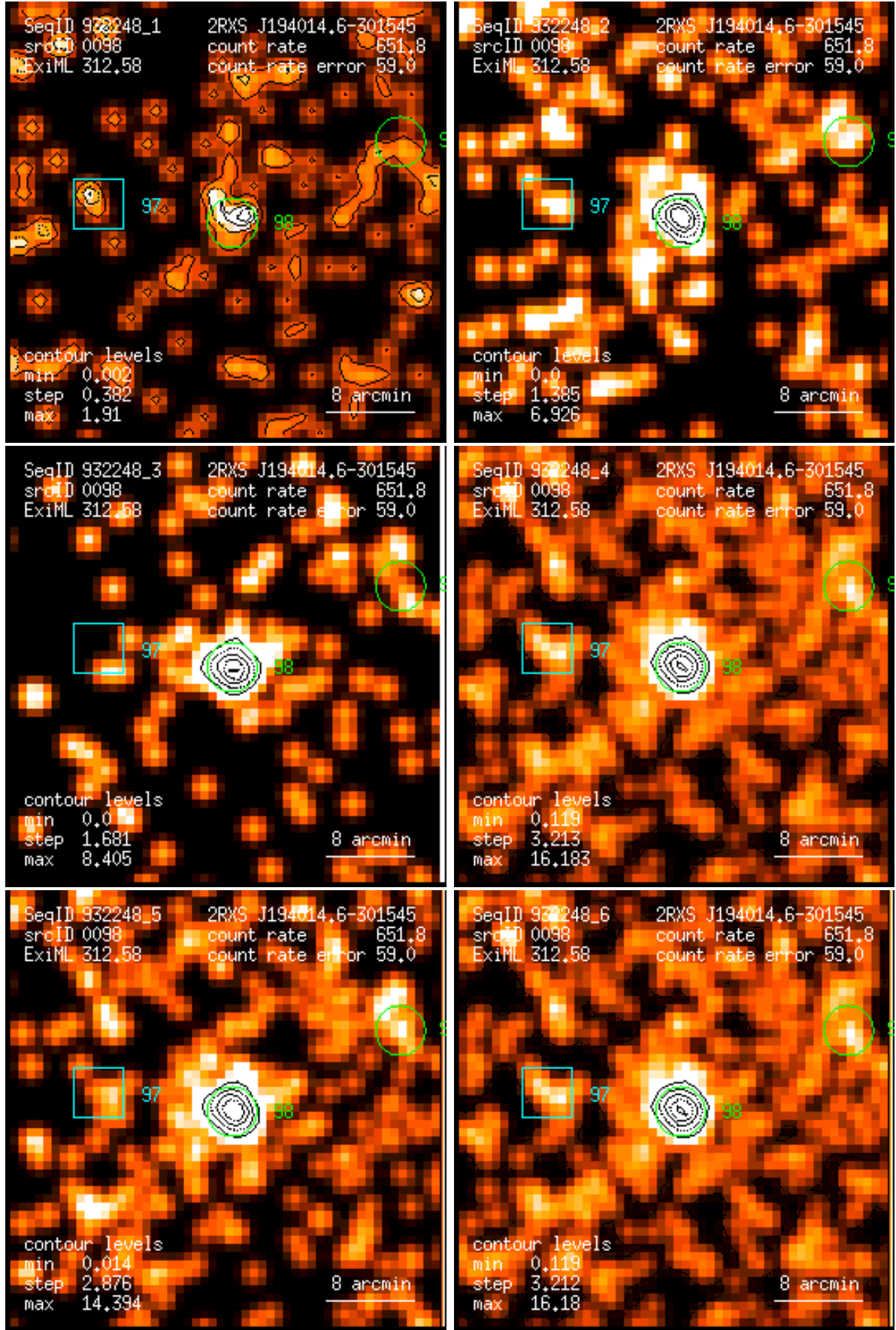
Figure 98: RASS 932248: detection 0098: band rate images, Gaussian filter: (1) PSPC channels 11 – 41, (2) 52 – 90, (3) 91 – 201, (4) 11 – 235, (5) 52 – 201, (6) 11 – 201. Broad band rates in counts/ks. Band rate contour levels in counts/ks/arcmin 2 .
