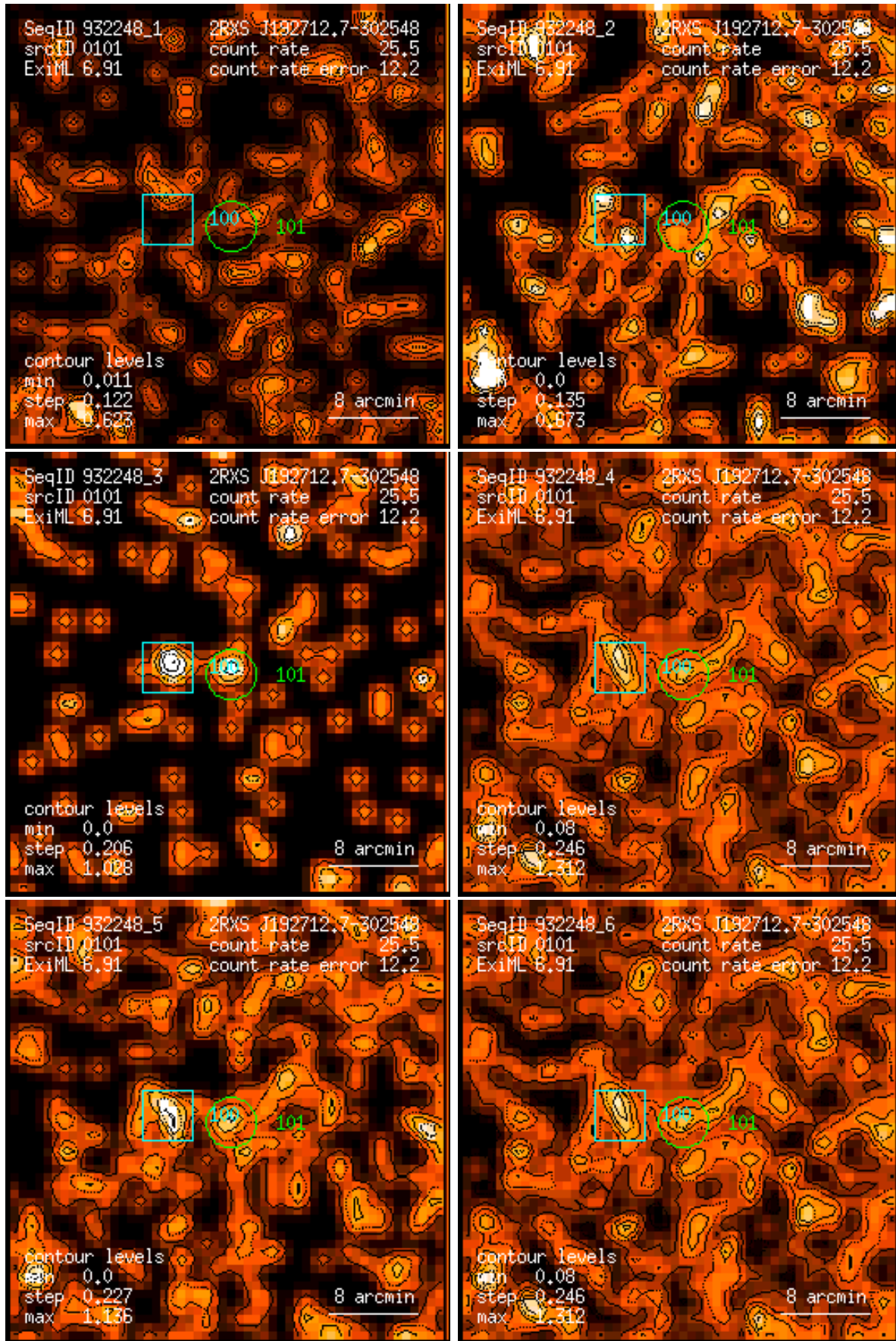
Figure 101: RASS 932248: detection 0101: band rate images, Gaussian filter: (1) PSPC channels 11 – 41, (2) 52 – 90, (3) 91 – 201, (4) 11 – 235, (5) 52 – 201, (6) 11 – 201. Broad band rates in counts/ks. Band rate contour levels in counts/ks/arcmin 2 .
