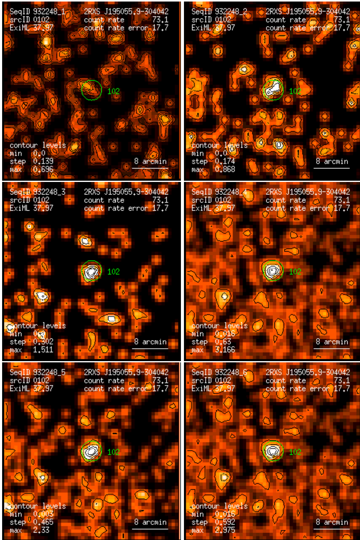
Figure 102: RASS 932248: detection 0102: band rate images, Gaussian filter: (1) PSPC channels 11 – 41, (2) 52 – 90, (3) 91 – 201, (4) 11 – 235, (5) 52 – 201, (6) 11 – 201. Broad band rates in counts/ks. Band rate contour levels in counts/ks/arcmin 2 .
