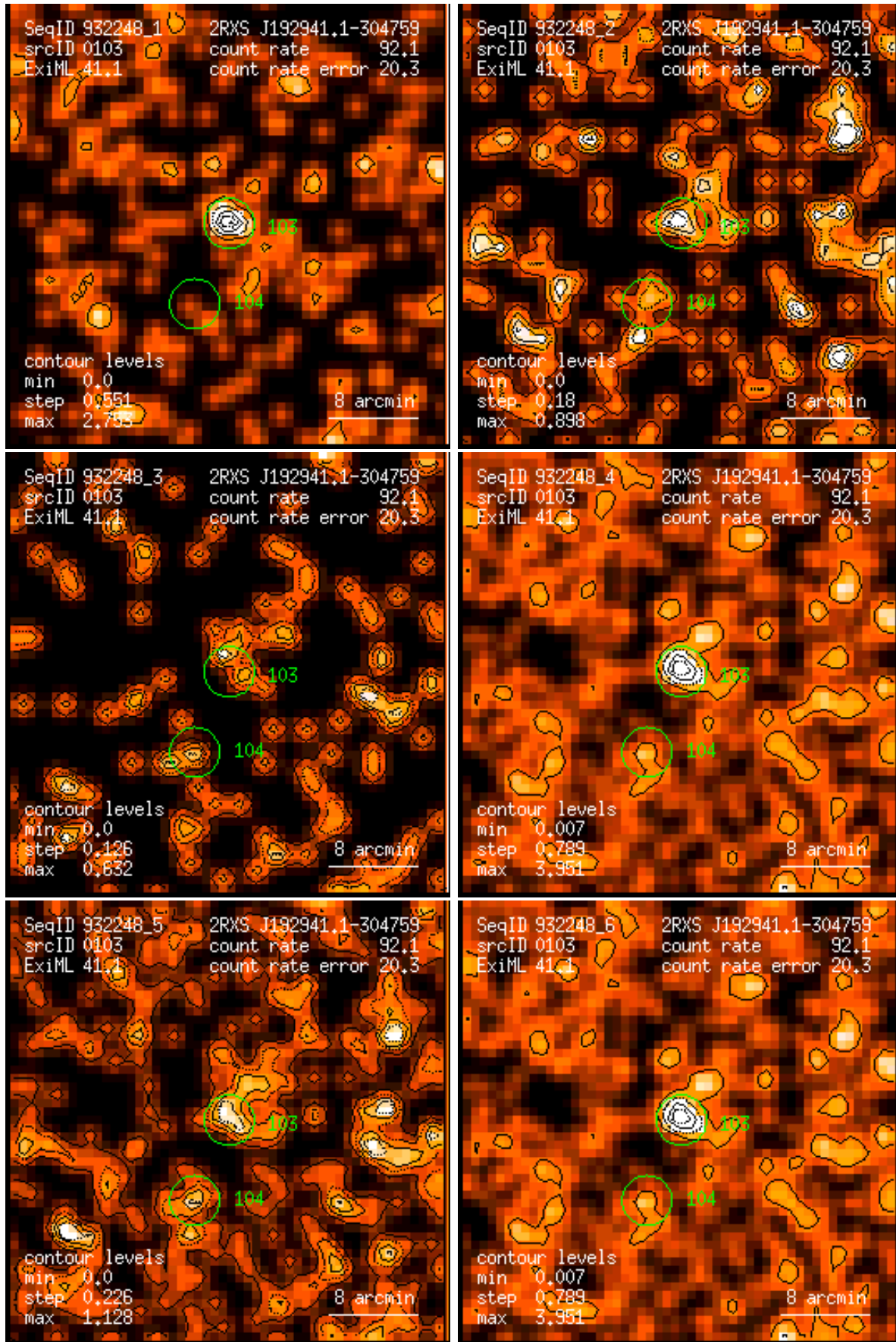
Figure 103: RASS 932248: detection 0103: band rate images, Gaussian filter: (1) PSPC channels 11 – 41, (2) 52 – 90, (3) 91 – 201, (4) 11 – 235, (5) 52 – 201, (6) 11 – 201. Broad band rates in counts/ks. Band rate contour levels in counts/ks/arcmin 2 .
