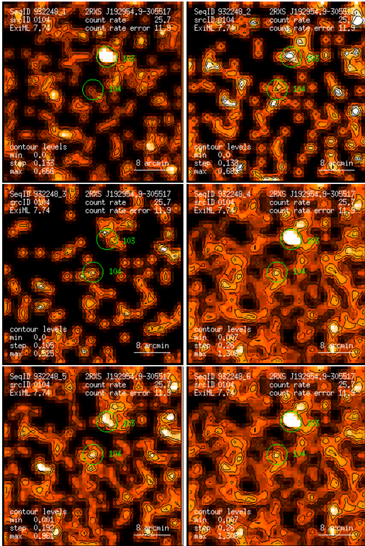
Figure 104: RASS 932248: detection 0104: band rate images, Gaussian filter: (1) PSPC channels 11 – 41, (2) 52 – 90, (3) 91 – 201, (4) 11 – 235, (5) 52 – 201, (6) 11 – 201. Broad band rates in counts/ks. Band rate contour levels in counts/ks/arcmin 2 .
