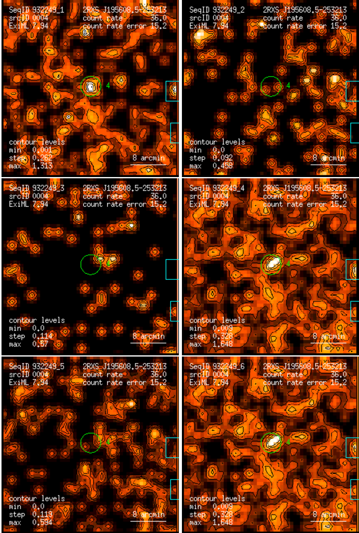
Figure 4: RASS 932249: detection 0004: band rate images, Gaussian filter: (1) PSPC channels 11 – 41, (2) 52 – 90, (3) 91 – 201, (4) 11 – 235, (5) 52 – 201, (6) 11 – 201. Broad band rates in counts/ks. Band rate contour levels in counts/ks/arcmin 2 .
