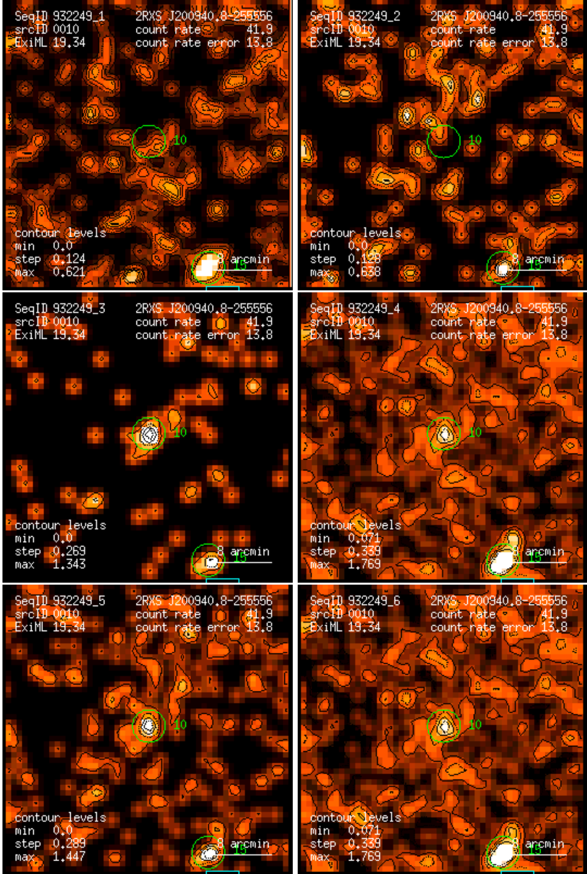
Figure 10: RASS 932249: detection 0010: band rate images, Gaussian filter: (1) PSPC channels 11 – 41, (2) 52 – 90, (3) 91 – 201, (4) 11 – 235, (5) 52 – 201, (6) 11 – 201. Broad band rates in counts/ks. Band rate contour levels in counts/ks/arcmin 2 .
