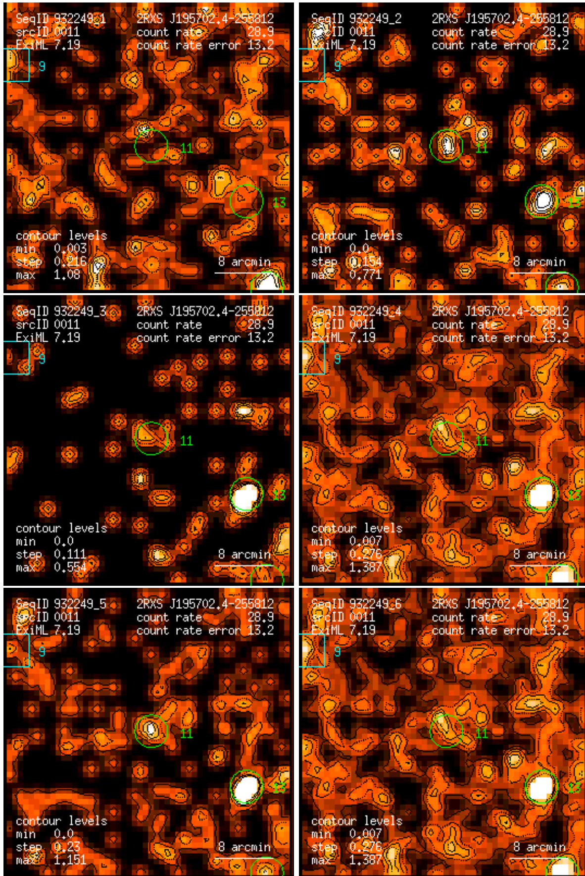
Figure 11: RASS 932249: detection 0011: band rate images, Gaussian filter: (1) PSPC channels 11 – 41, (2) 52 – 90, (3) 91 – 201, (4) 11 – 235, (5) 52 – 201, (6) 11 – 201. Broad band rates in counts/ks. Band rate contour levels in counts/ks/arcmin 2 .
