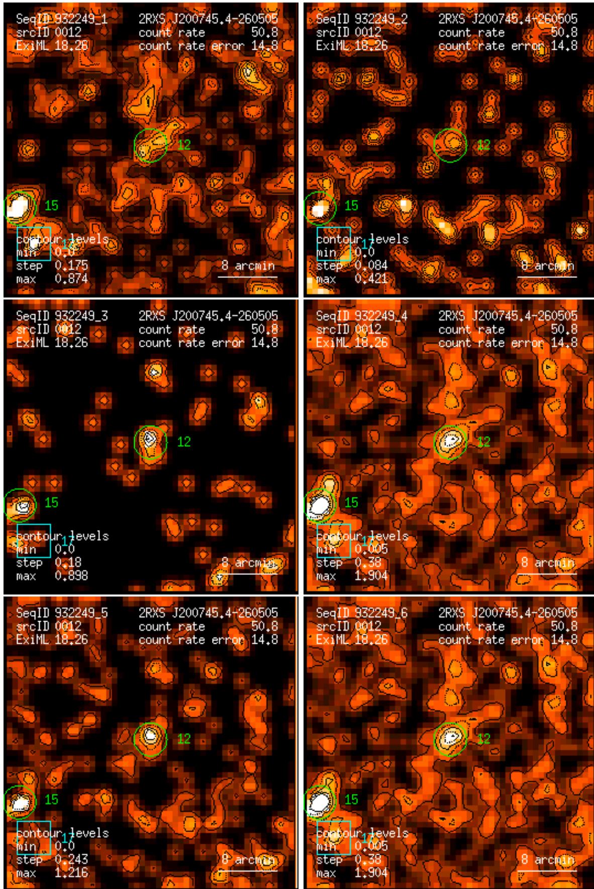
Figure 12: RASS 932249: detection 0012: band rate images, Gaussian filter: (1) PSPC channels 11 – 41, (2) 52 – 90, (3) 91 – 201, (4) 11 – 235, (5) 52 – 201, (6) 11 – 201. Broad band rates in counts/ks. Band rate contour levels in counts/ks/arcmin 2 .
