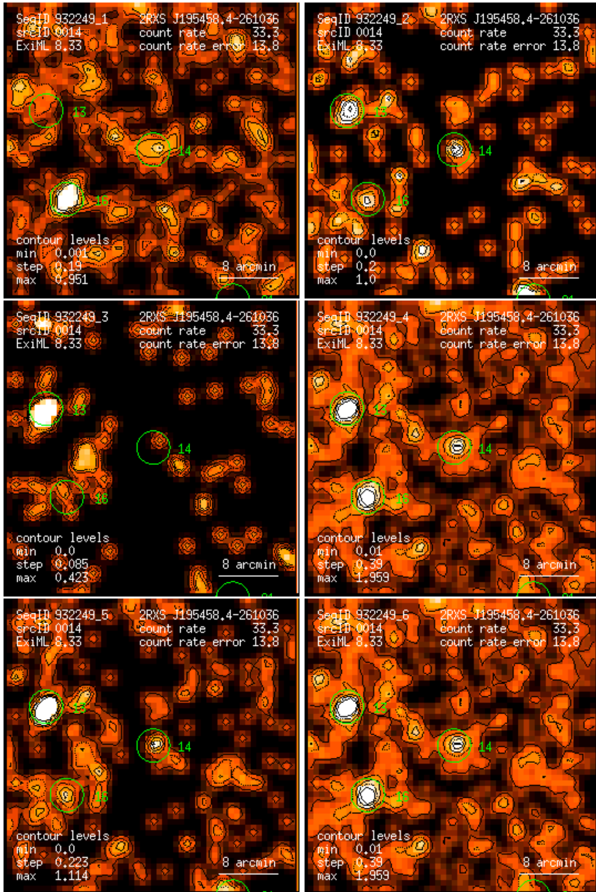
Figure 14: RASS 932249: detection 0014: band rate images, Gaussian filter: (1) PSPC channels 11 – 41, (2) 52 – 90, (3) 91 – 201, (4) 11 – 235, (5) 52 – 201, (6) 11 – 201. Broad band rates in counts/ks. Band rate contour levels in counts/ks/arcmin 2 .
