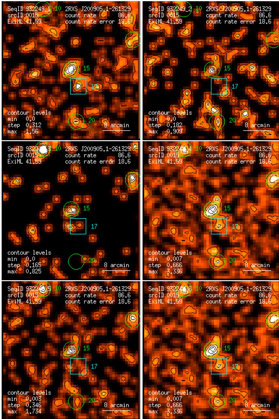
Figure 15: RASS 932249: detection 0015: band rate images, Gaussian filter: (1) PSPC channels 11 – 41, (2) 52 – 90, (3) 91 – 201, (4) 11 – 235, (5) 52 – 201, (6) 11 – 201. Broad band rates in counts/ks. Band rate contour levels in counts/ks/arcmin 2 .
