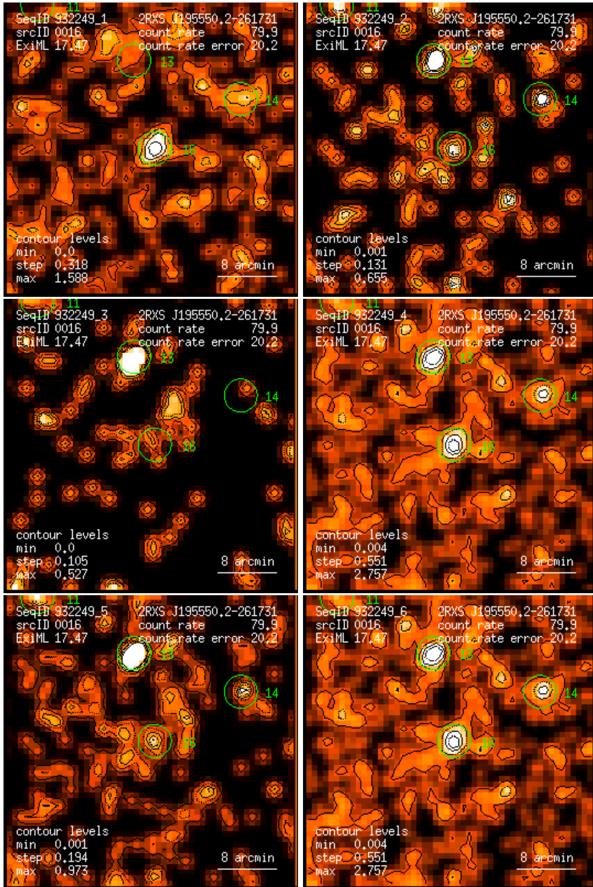
Figure 16: RASS 932249: detection 0016: band rate images, Gaussian filter: (1) PSPC channels 11 – 41, (2) 52 – 90, (3) 91 – 201, (4) 11 – 235, (5) 52 – 201, (6) 11 – 201. Broad band rates in counts/ks. Band rate contour levels in counts/ks/arcmin 2 .
