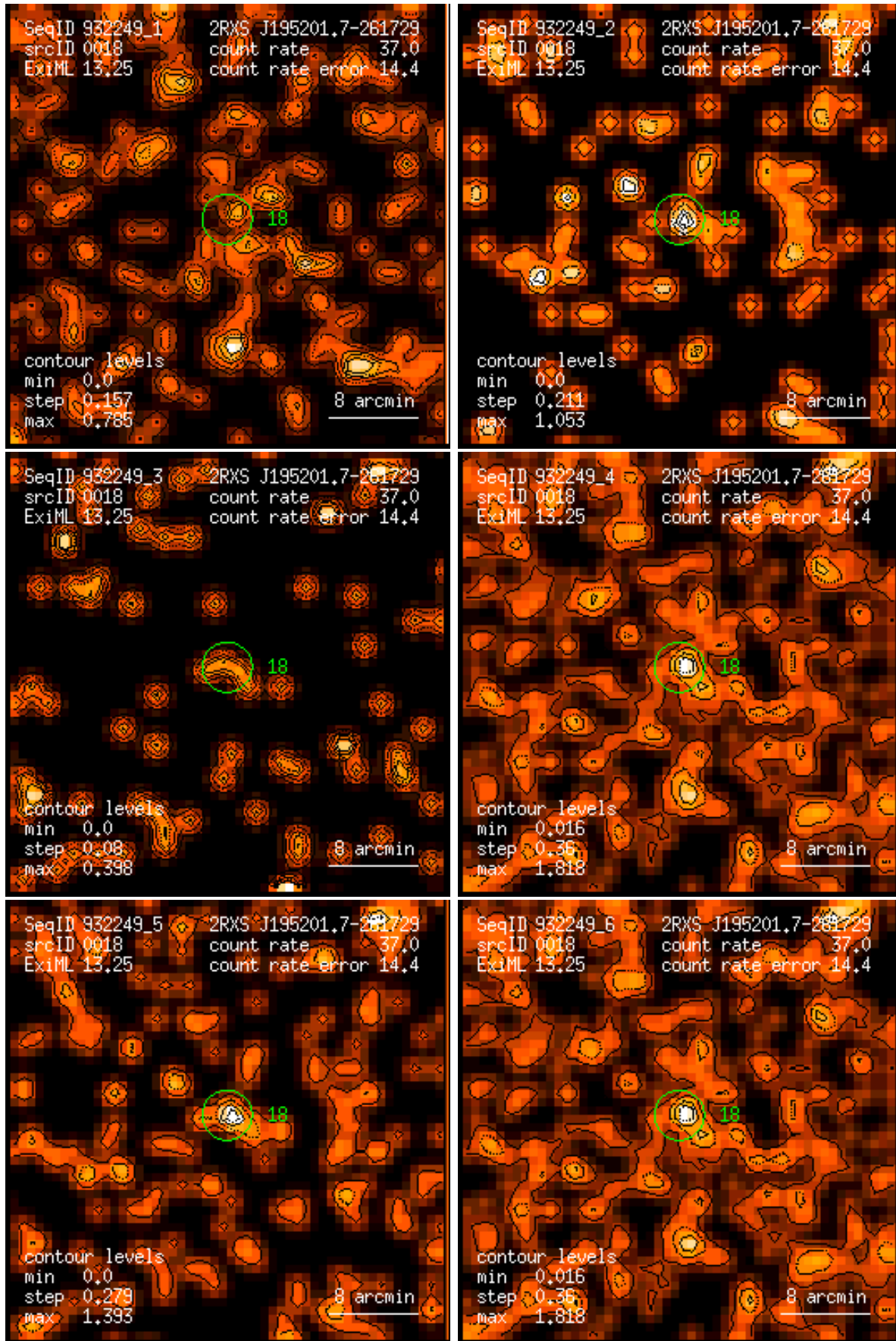
Figure 18: RASS 932249: detection 0018: band rate images, Gaussian filter: (1) PSPC channels 11 – 41, (2) 52 – 90, (3) 91 – 201, (4) 11 – 235, (5) 52 – 201, (6) 11 – 201. Broad band rates in counts/ks. Band rate contour levels in counts/ks/arcmin 2 .
