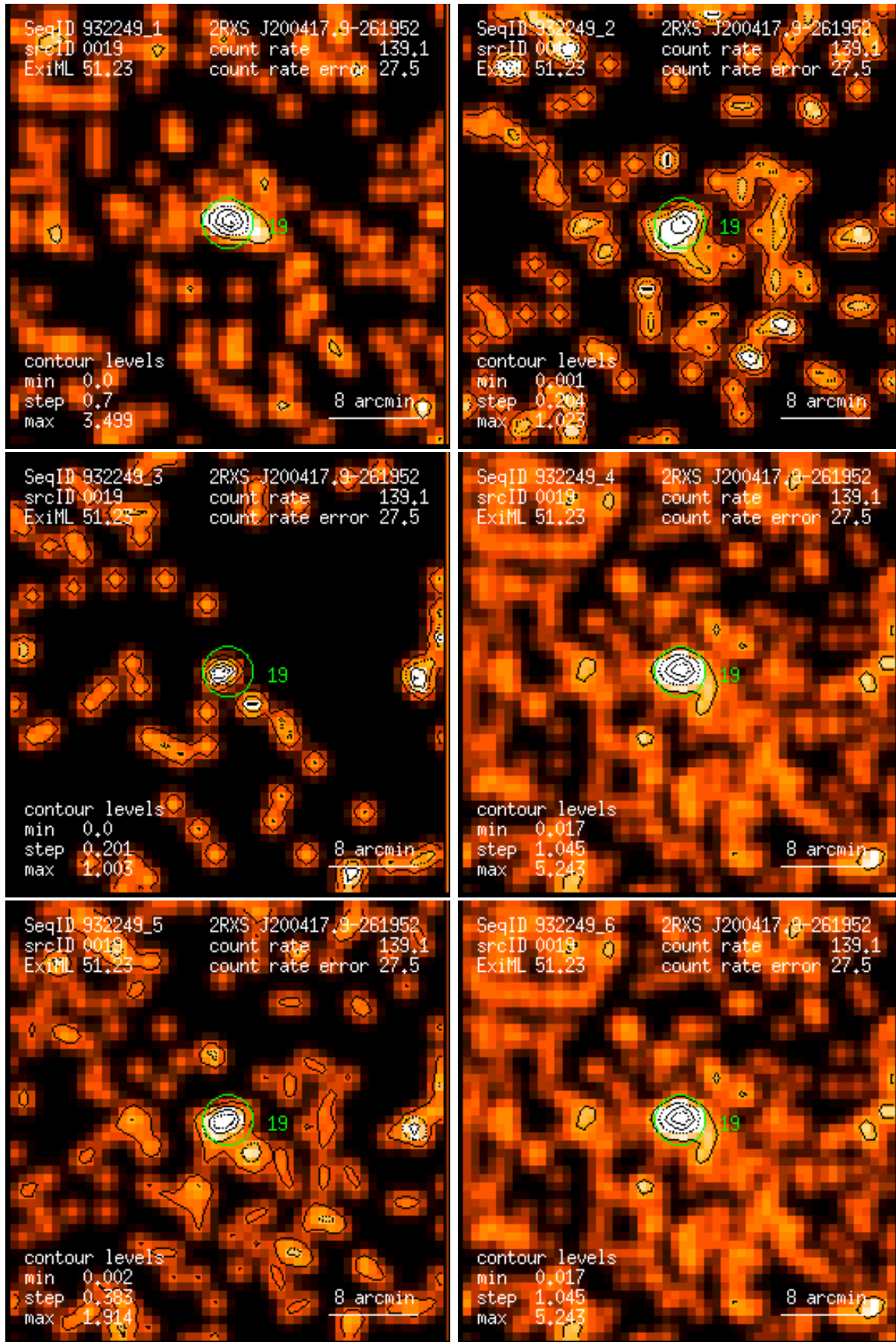
Figure 19: RASS 932249: detection 0019: band rate images, Gaussian filter: (1) PSPC channels 11 – 41, (2) 52 – 90, (3) 91 – 201, (4) 11 – 235, (5) 52 – 201, (6) 11 – 201. Broad band rates in counts/ks. Band rate contour levels in counts/ks/arcmin 2 .
