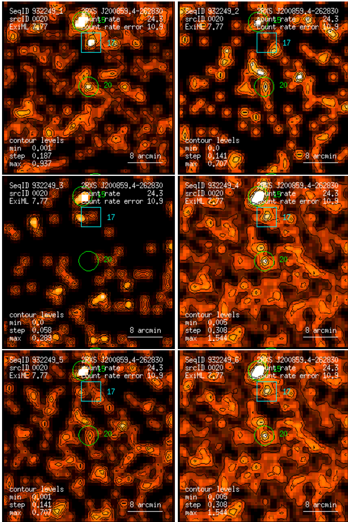
Figure 20: RASS 932249: detection 0020: band rate images, Gaussian filter: (1) PSPC channels 11 – 41, (2) 52 – 90, (3) 91 – 201, (4) 11 – 235, (5) 52 – 201, (6) 11 – 201. Broad band rates in counts/ks. Band rate contour levels in counts/ks/arcmin 2 .
