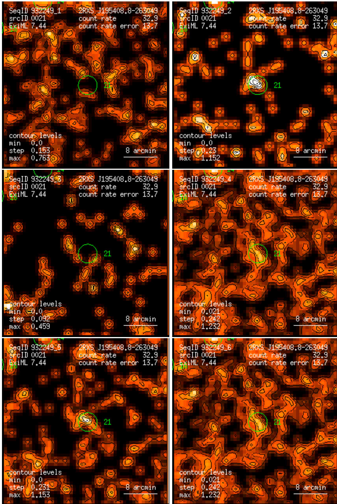
Figure 21: RASS 932249: detection 0021: band rate images, Gaussian filter: (1) PSPC channels 11 – 41, (2) 52 – 90, (3) 91 – 201, (4) 11 – 235, (5) 52 – 201, (6) 11 – 201. Broad band rates in counts/ks. Band rate contour levels in counts/ks/arcmin 2 .
