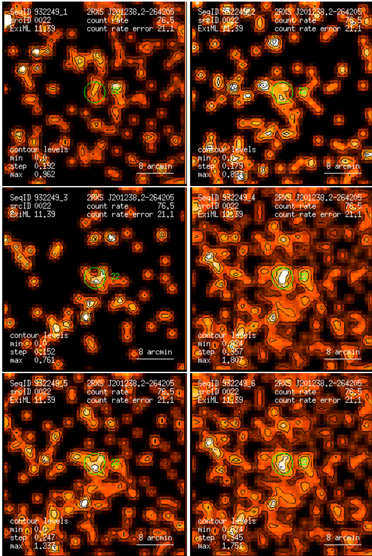
Figure 22: RASS 932249: detection 0022: band rate images, Gaussian filter: (1) PSPC channels 11 – 41, (2) 52 – 90, (3) 91 – 201, (4) 11 – 235, (5) 52 – 201, (6) 11 – 201. Broad band rates in counts/ks. Band rate contour levels in counts/ks/arcmin 2 .
