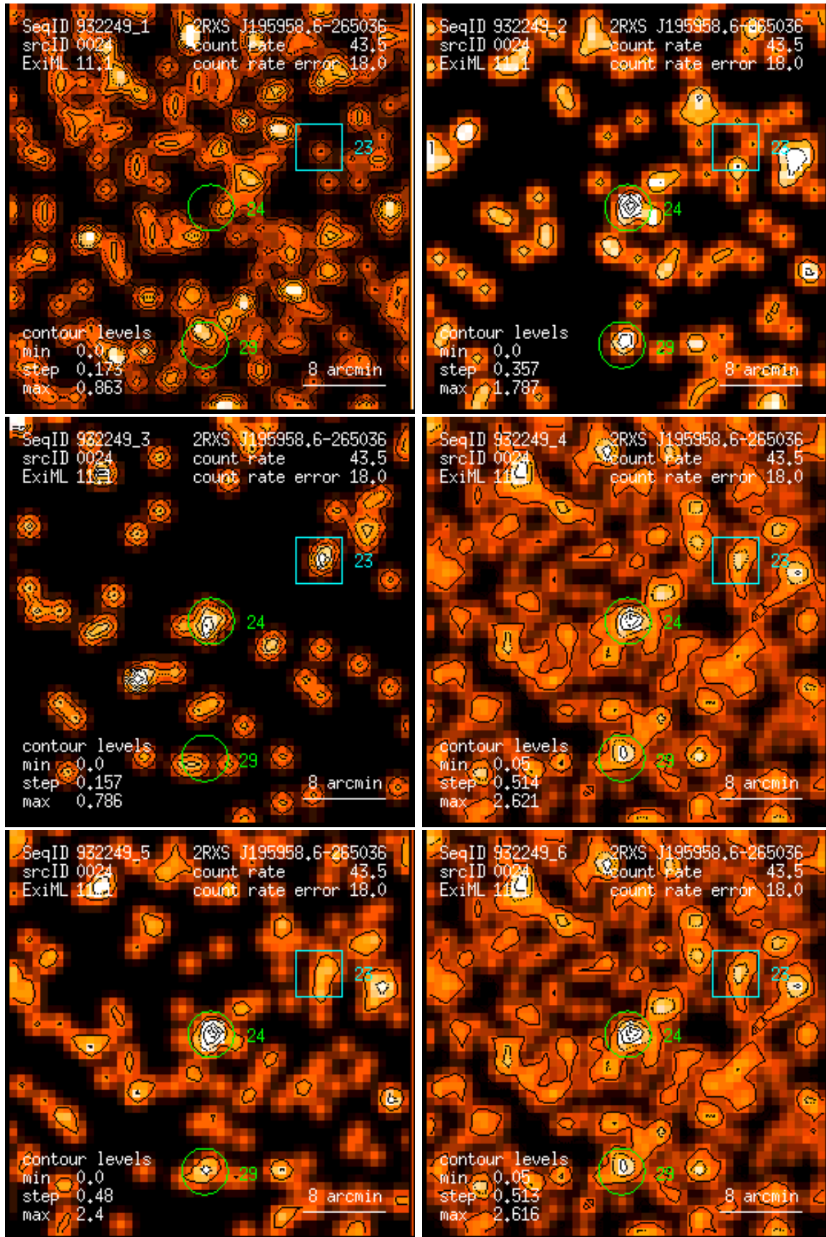
Figure 24: RASS 932249: detection 0024: band rate images, Gaussian filter: (1) PSPC channels 11 – 41, (2) 52 – 90, (3) 91 – 201, (4) 11 – 235, (5) 52 – 201, (6) 11 – 201. Broad band rates in counts/ks. Band rate contour levels in counts/ks/arcmin 2 .
