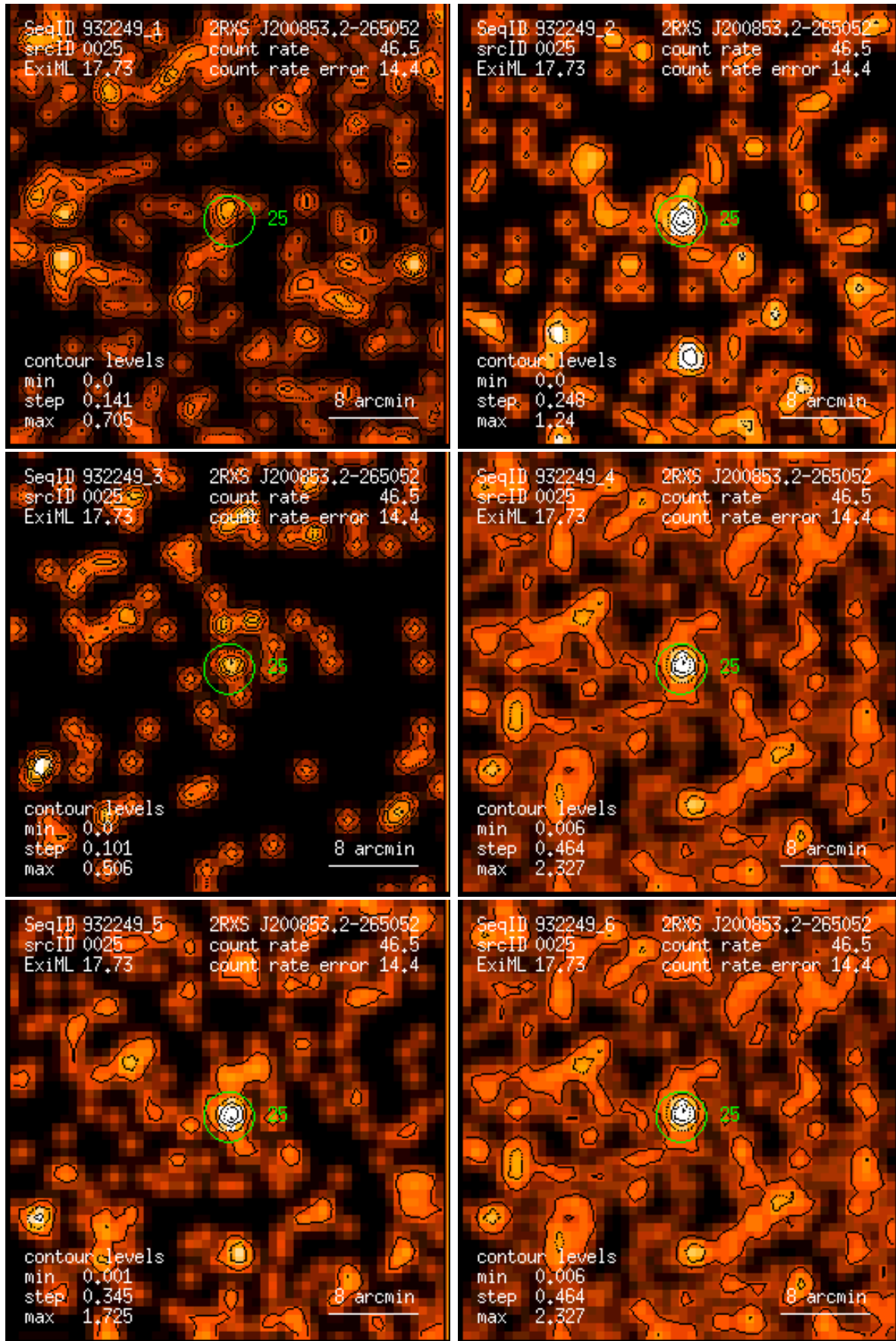
Figure 25: RASS 932249: detection 0025: band rate images, Gaussian filter: (1) PSPC channels 11 – 41, (2) 52 – 90, (3) 91 – 201, (4) 11 – 235, (5) 52 – 201, (6) 11 – 201. Broad band rates in counts/ks. Band rate contour levels in counts/ks/arcmin 2 .
