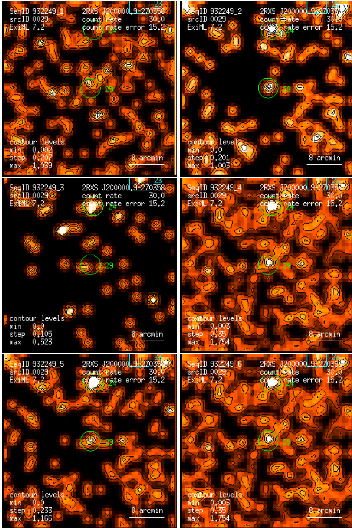
Figure 29: RASS 932249: detection 0029: band rate images, Gaussian filter: (1) PSPC channels 11 – 41, (2) 52 – 90, (3) 91 – 201, (4) 11 – 235, (5) 52 – 201, (6) 11 – 201. Broad band rates in counts/ks. Band rate contour levels in counts/ks/arcmin 2 .
