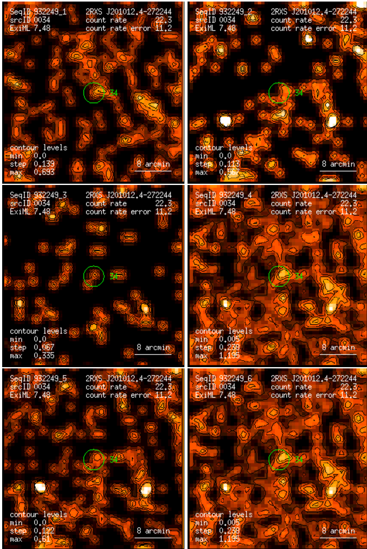
Figure 34: RASS 932249: detection 0034: band rate images, Gaussian filter: (1) PSPC channels 11 – 41, (2) 52 – 90, (3) 91 – 201, (4) 11 – 235, (5) 52 – 201, (6) 11 – 201. Broad band rates in counts/ks. Band rate contour levels in counts/ks/arcmin 2 .
