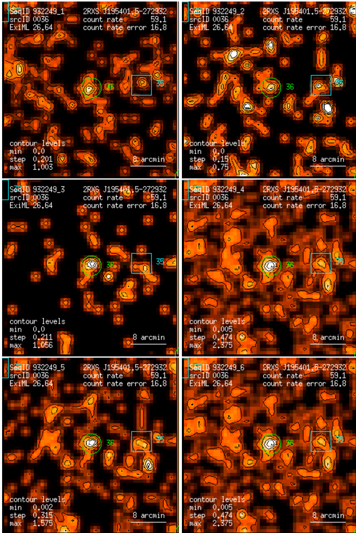
Figure 36: RASS 932249: detection 0036: band rate images, Gaussian filter: (1) PSPC channels 11 – 41, (2) 52 – 90, (3) 91 – 201, (4) 11 – 235, (5) 52 – 201, (6) 11 – 201. Broad band rates in counts/ks. Band rate contour levels in counts/ks/arcmin 2 .
