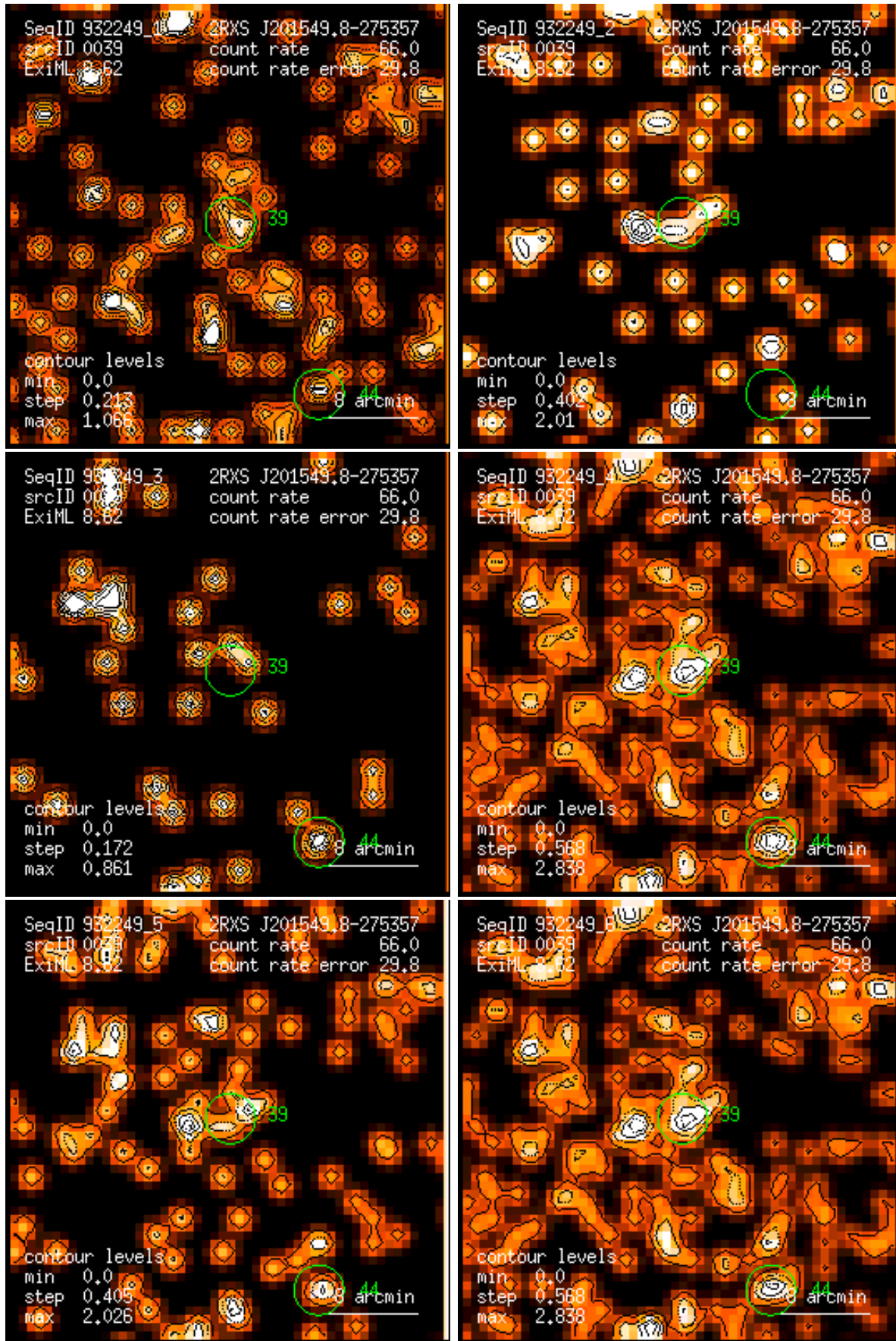
Figure 39: RASS 932249: detection 0039: band rate images, Gaussian filter: (1) PSPC channels 11 – 41, (2) 52 – 90, (3) 91 – 201, (4) 11 – 235, (5) 52 – 201, (6) 11 – 201. Broad band rates in counts/ks. Band rate contour levels in counts/ks/arcmin 2 .
