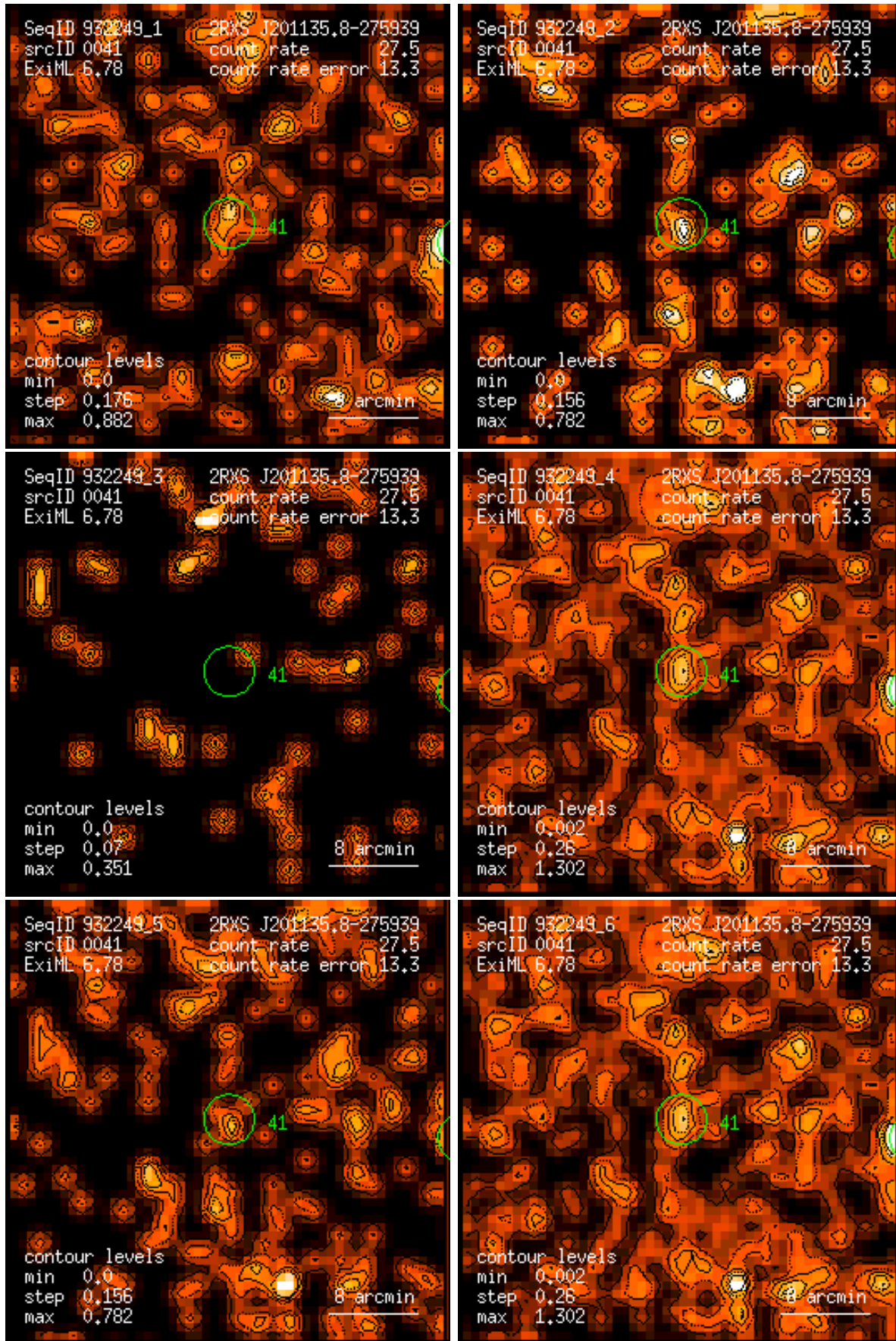
Figure 41: RASS 932249: detection 0041: band rate images, Gaussian filter: (1) PSPC channels 11 – 41, (2) 52 – 90, (3) 91 – 201, (4) 11 – 235, (5) 52 – 201, (6) 11 – 201. Broad band rates in counts/ks. Band rate contour levels in counts/ks/arcmin 2 .
