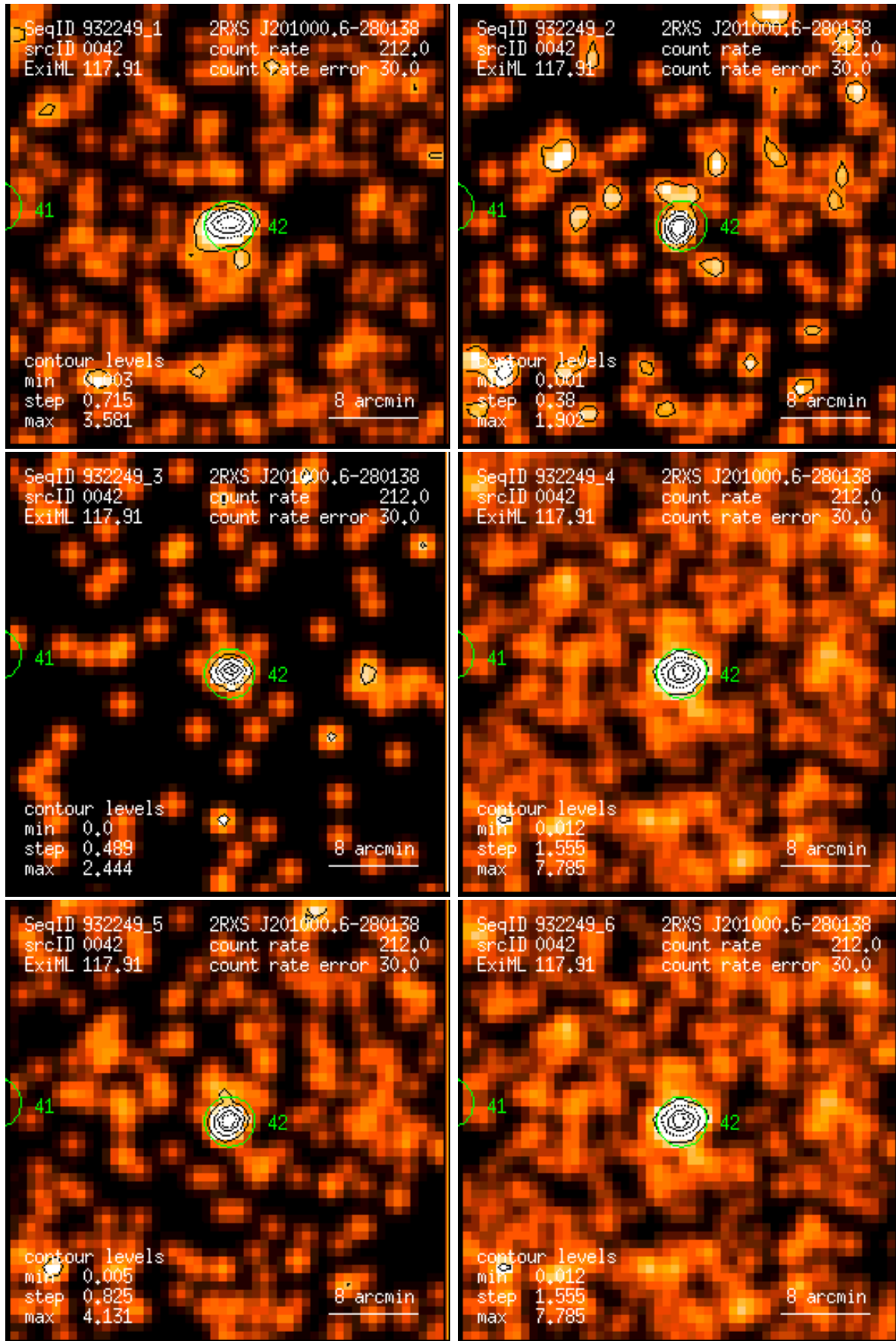
Figure 42: RASS 932249: detection 0042: band rate images, Gaussian filter: (1) PSPC channels 11 – 41, (2) 52 – 90, (3) 91 – 201, (4) 11 – 235, (5) 52 – 201, (6) 11 – 201. Broad band rates in counts/ks. Band rate contour levels in counts/ks/arcmin 2 .
