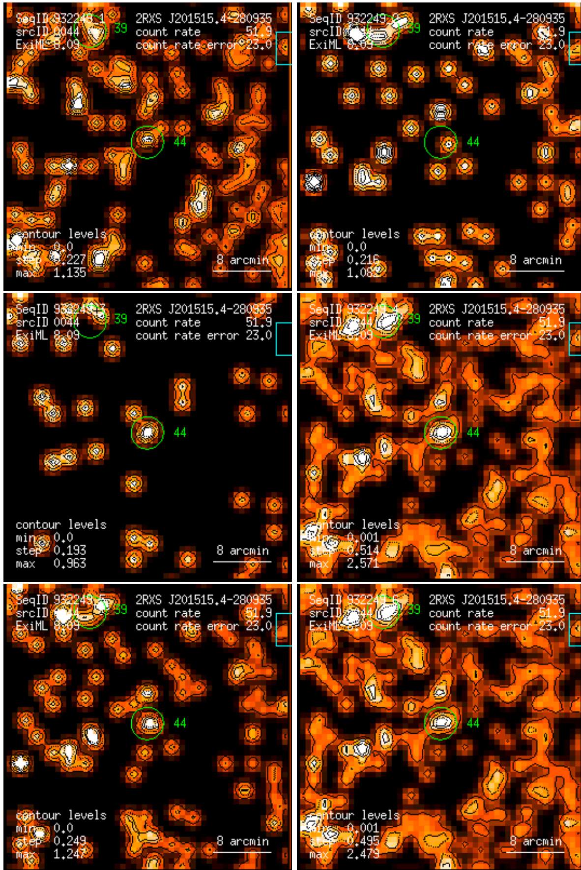
Figure 44: RASS 932249: detection 0044: band rate images, Gaussian filter: (1) PSPC channels 11 – 41, (2) 52 – 90, (3) 91 – 201, (4) 11 – 235, (5) 52 – 201, (6) 11 – 201. Broad band rates in counts/ks. Band rate contour levels in counts/ks/arcmin 2 .
