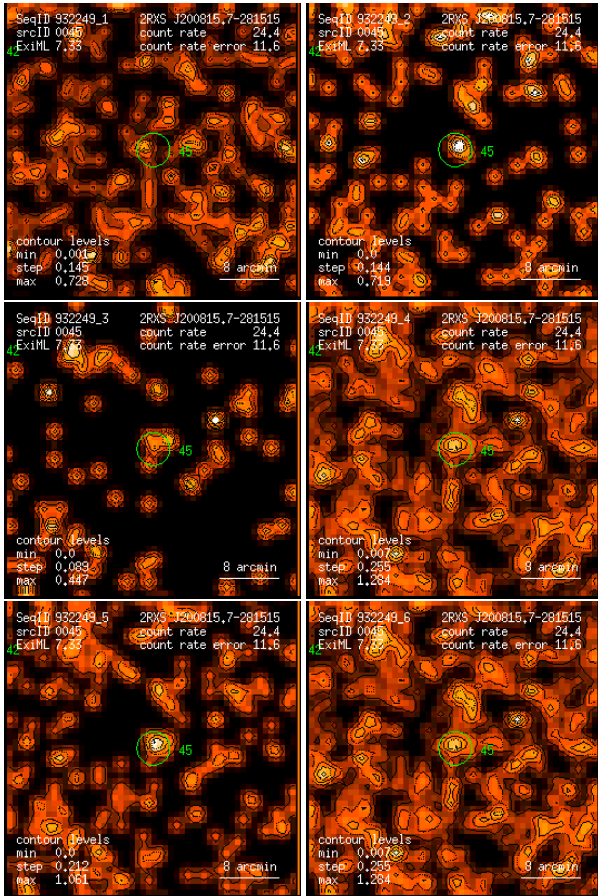
Figure 45: RASS 932249: detection 0045: band rate images, Gaussian filter: (1) PSPC channels 11 – 41, (2) 52 – 90, (3) 91 – 201, (4) 11 – 235, (5) 52 – 201, (6) 11 – 201. Broad band rates in counts/ks. Band rate contour levels in counts/ks/arcmin 2 .
