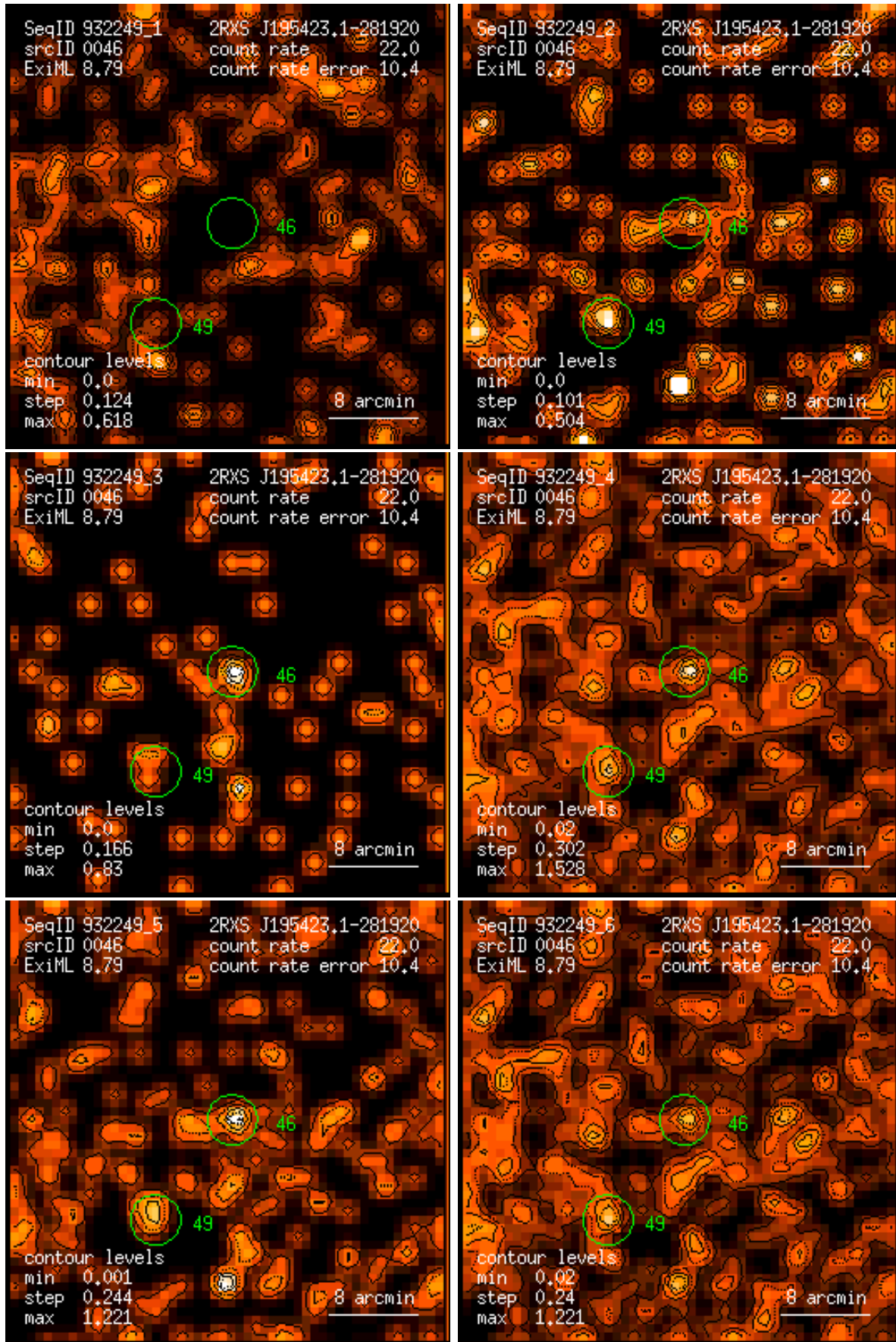
Figure 46: RASS 932249: detection 0046: band rate images, Gaussian filter: (1) PSPC channels 11 – 41, (2) 52 – 90, (3) 91 – 201, (4) 11 – 235, (5) 52 – 201, (6) 11 – 201. Broad band rates in counts/ks. Band rate contour levels in counts/ks/arcmin 2 .
