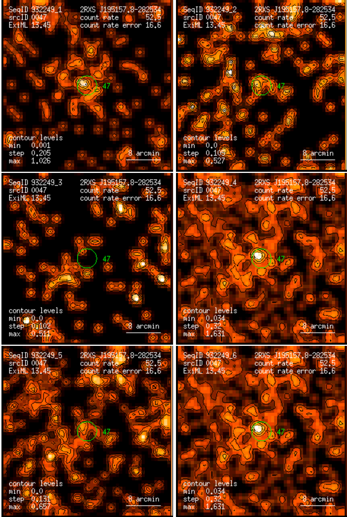
Figure 47: RASS 932249: detection 0047: band rate images, Gaussian filter: (1) PSPC channels 11 – 41, (2) 52 – 90, (3) 91 – 201, (4) 11 – 235, (5) 52 – 201, (6) 11 – 201. Broad band rates in counts/ks. Band rate contour levels in counts/ks/arcmin 2 .
