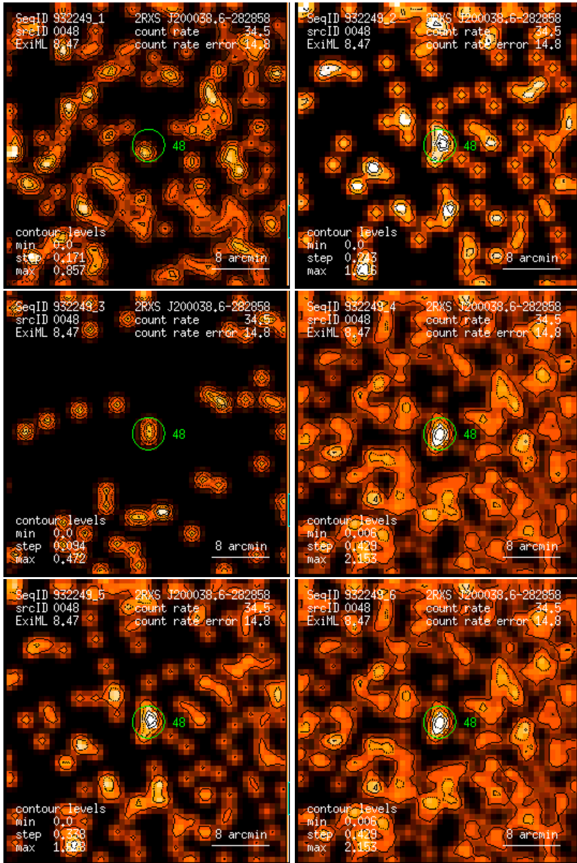
Figure 48: RASS 932249: detection 0048: band rate images, Gaussian filter: (1) PSPC channels 11 – 41, (2) 52 – 90, (3) 91 – 201, (4) 11 – 235, (5) 52 – 201, (6) 11 – 201. Broad band rates in counts/ks. Band rate contour levels in counts/ks/arcmin 2 .
