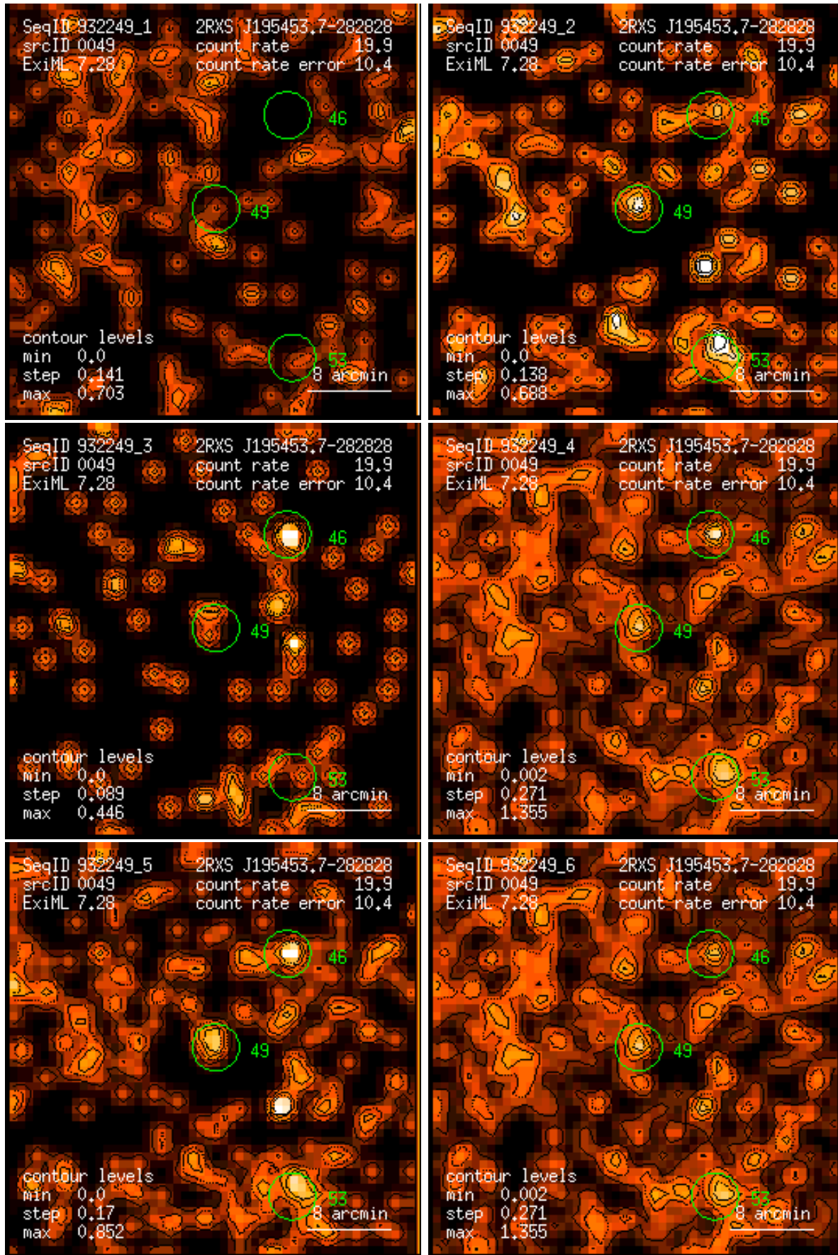
Figure 49: RASS 932249: detection 0049: band rate images, Gaussian filter: (1) PSPC channels 11 – 41, (2) 52 – 90, (3) 91 – 201, (4) 11 – 235, (5) 52 – 201, (6) 11 – 201. Broad band rates in counts/ks. Band rate contour levels in counts/ks/arcmin 2 .
