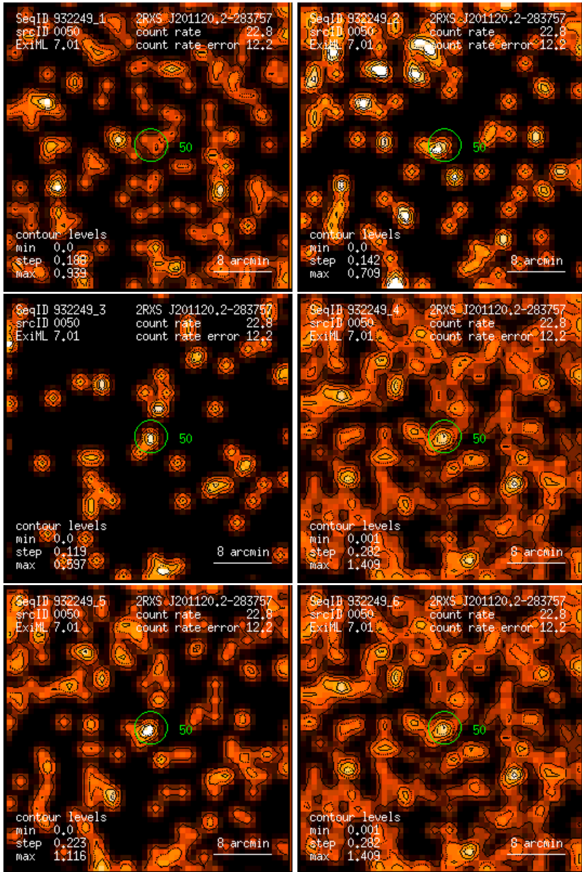
Figure 50: RASS 932249: detection 0050: band rate images, Gaussian filter: (1) PSPC channels 11 – 41, (2) 52 – 90, (3) 91 – 201, (4) 11 – 235, (5) 52 – 201, (6) 11 – 201. Broad band rates in counts/ks. Band rate contour levels in counts/ks/arcmin 2 .
