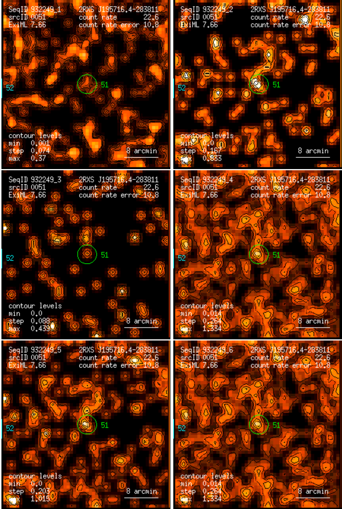
Figure 51: RASS 932249: detection 0051: band rate images, Gaussian filter: (1) PSPC channels 11 – 41, (2) 52 – 90, (3) 91 – 201, (4) 11 – 235, (5) 52 – 201, (6) 11 – 201. Broad band rates in counts/ks. Band rate contour levels in counts/ks/arcmin 2 .
